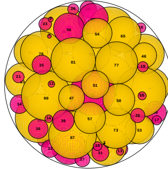
N = 91 91 spheres in a sphere
