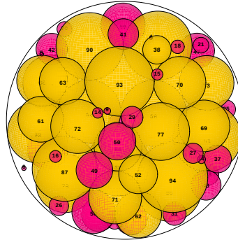
N = 94 94 spheres in a sphere
