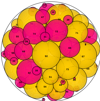
N = 95 95 spheres in a sphere
