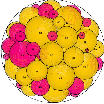
N = 86 86 spheres in a sphere
