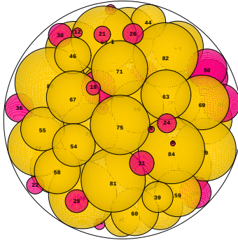
N = 90 90 spheres in a sphere
