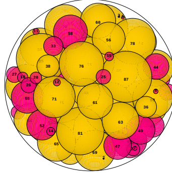
N = 88 88 spheres in a sphere
