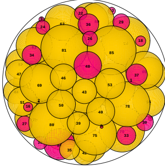
N = 87 87 spheres in a sphere
