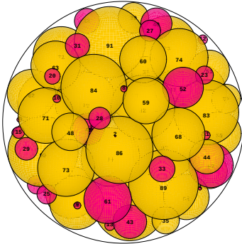
N = 92 92 spheres in a sphere
