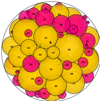
N = 96 96 spheres in a sphere
