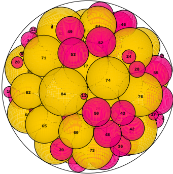
N = 89 89 spheres in a sphere
