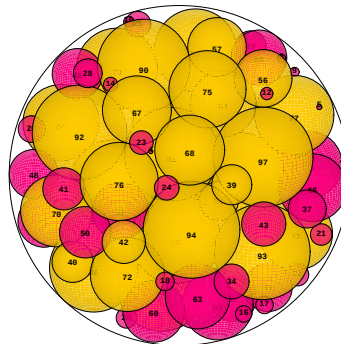
N = 97 97 spheres in a sphere
