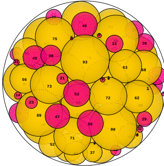
N = 93 93 spheres in a sphere
