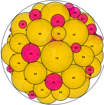
N = 77 77 spheres in a sphere
