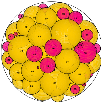
N = 83 83 spheres in a sphere
