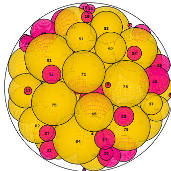
N = 85 85 spheres in a sphere
