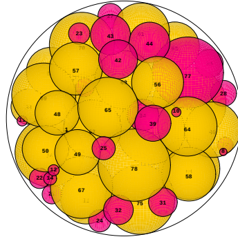
N = 79 79 spheres in a sphere
