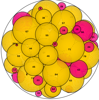
N = 74 74 spheres in a sphere
