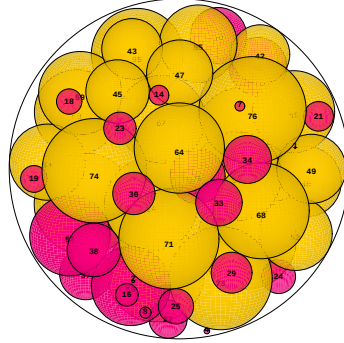
N = 76 76 spheres in a sphere
