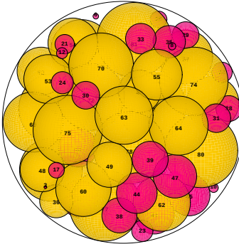
N = 81 81 spheres in a sphere
