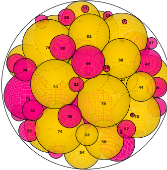
N = 78 78 spheres in a sphere
