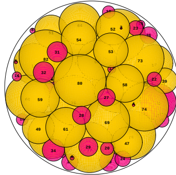
N = 82 82 spheres in a sphere
