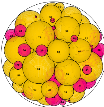
N = 84 84 spheres in a sphere
