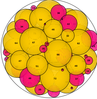
N = 75 75 spheres in a sphere
