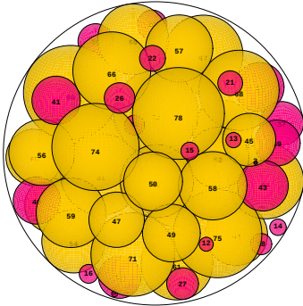
N = 80 80 spheres in a sphere
