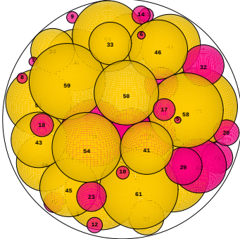
N = 62 62 spheres in a sphere
