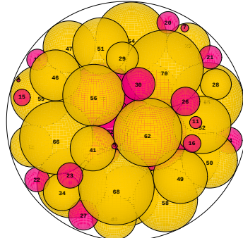
N = 70 70 spheres in a sphere
