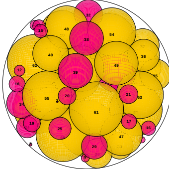
N = 63 63 spheres in a sphere
