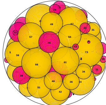
N = 73 73 spheres in a sphere
