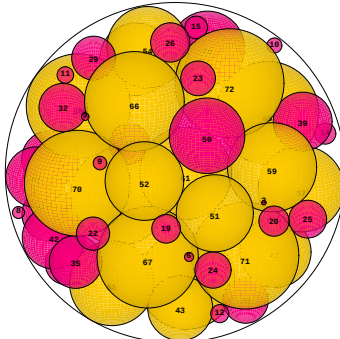
N = 72 72 spheres in a sphere
