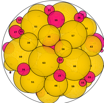
N = 69 69 spheres in a sphere
