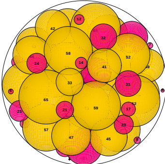
N = 65 65 spheres in a sphere
