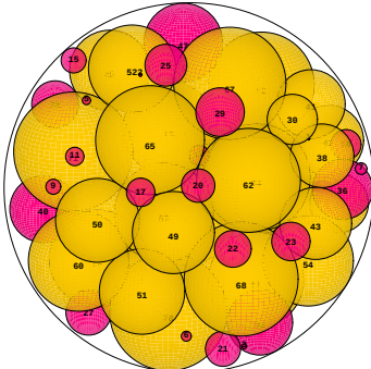
N = 71 71 spheres in a sphere
