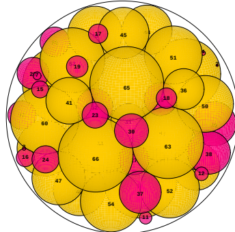
N = 67 67 spheres in a sphere
