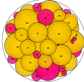
N = 64 64 spheres in a sphere
