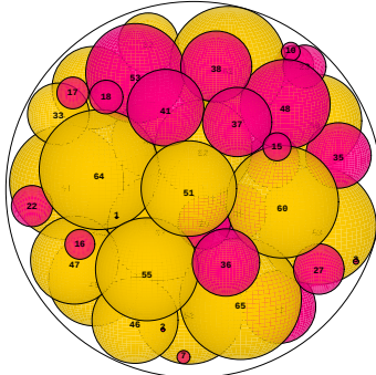
N = 66 66 spheres in a sphere
