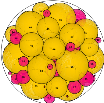
N = 68 68 spheres in a sphere
