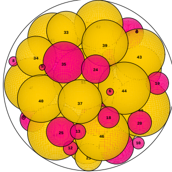
N = 51 51 spheres in a sphere
