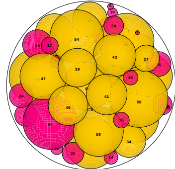
N = 58 58 spheres in a sphere
