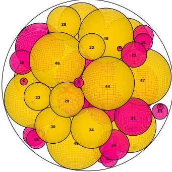
N = 50 50 spheres in a sphere
