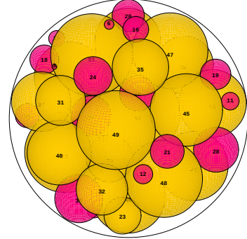
N = 52 52 spheres in a sphere
