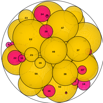
N = 53 53 spheres in a sphere
