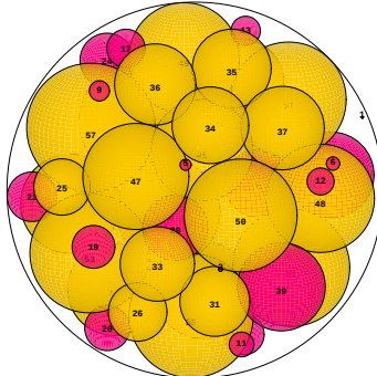
N = 57 57 spheres in a sphere
