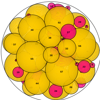
N = 59 59 spheres in a sphere
