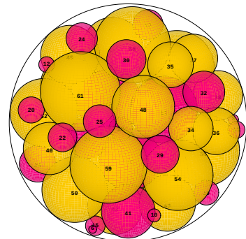
N = 61 61 spheres in a sphere
