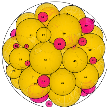
N = 60 60 spheres in a sphere
