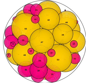
N = 55 55 spheres in a sphere
