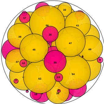
N = 56 56 spheres in a sphere
