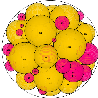
N = 54 54 spheres in a sphere
