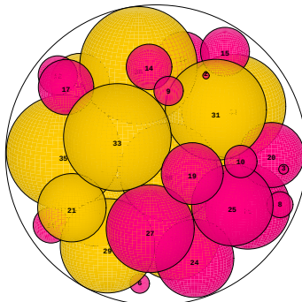
N = 36 36 spheres in a sphere
