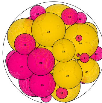
N = 37 37 spheres in a sphere
