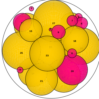
N = 27 27 spheres in a sphere
