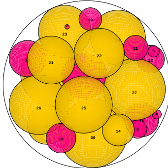
N = 30 30 spheres in a sphere
