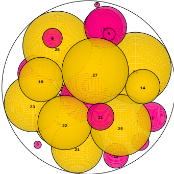
N = 29 29 spheres in a sphere
