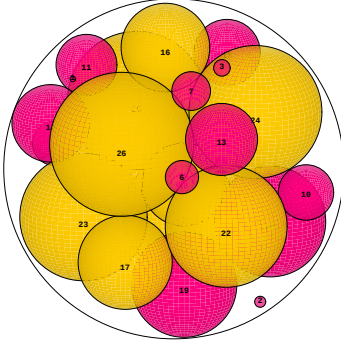
N = 26 26 spheres in a sphere
