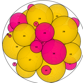
N = 34 34 spheres in a sphere
