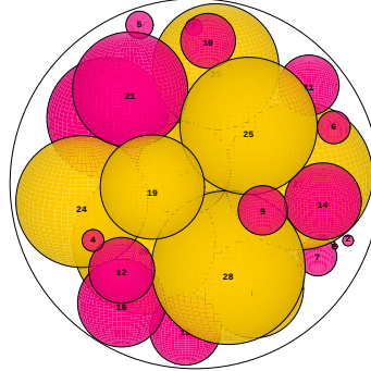
N = 28 28 spheres in a sphere
