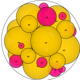
N = 33 33 spheres in a sphere
