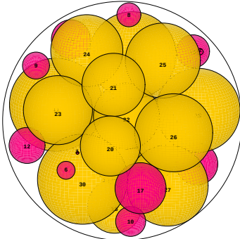
N = 32 32 spheres in a sphere
