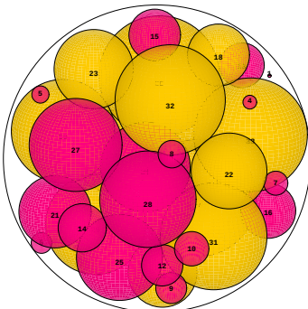
N = 35 35 spheres in a sphere
