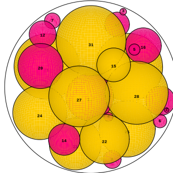
N = 31 31 spheres in a sphere
