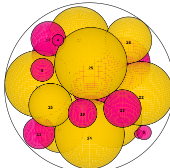
N = 25 25 spheres in a sphere
