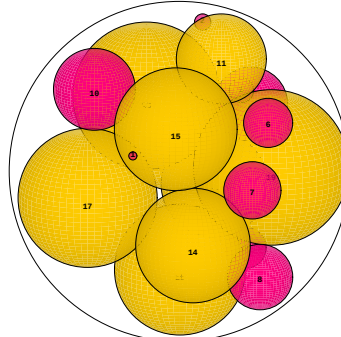
N = 19 19 spheres in a sphere
