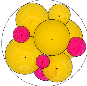
N = 15 15 spheres in a sphere
