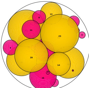
N = 23 23 spheres in a sphere
