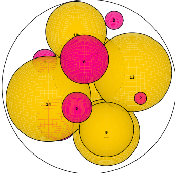
N = 14 14 spheres in a sphere
