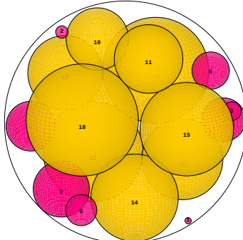
N = 18 18 spheres in a sphere
