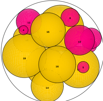
N = 20 20 spheres in a sphere
