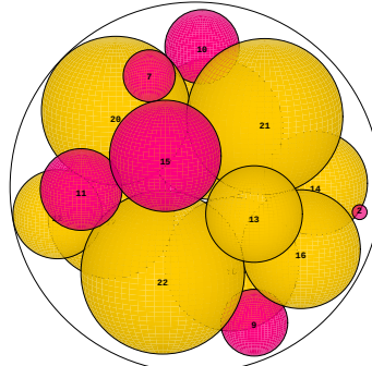
N = 22 22 spheres in a sphere
