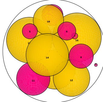
N = 16 16 spheres in a sphere
