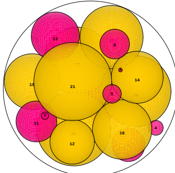
N = 21 21 spheres in a sphere
