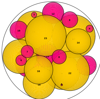
N = 24 24 spheres in a sphere
