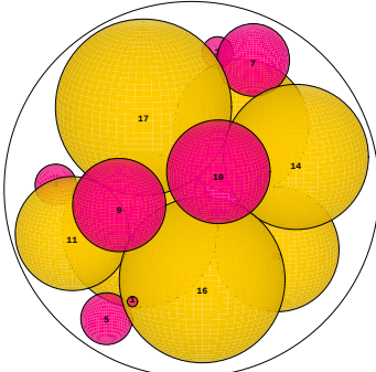
N = 17 17 spheres in a sphere
