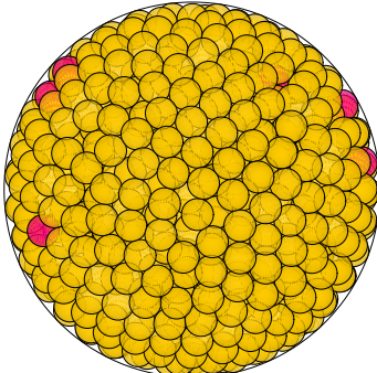
N = 991 991 spheres in a sphere
