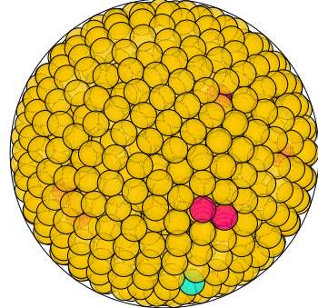
N = 987 987 spheres in a sphere
