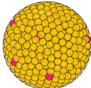
N = 996 996 spheres in a sphere
