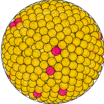
N = 985 985 spheres in a sphere
