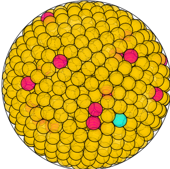
N = 988 988 spheres in a sphere
