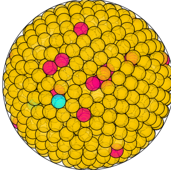
N = 986 986 spheres in a sphere
