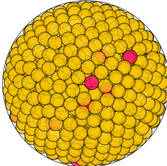
N = 989 989 spheres in a sphere
