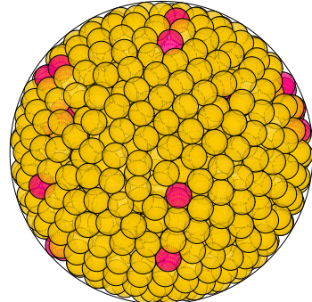
N = 990 990 spheres in a sphere
