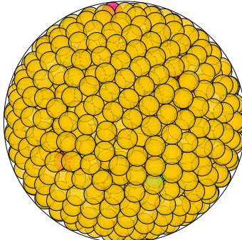
N = 992 992 spheres in a sphere
