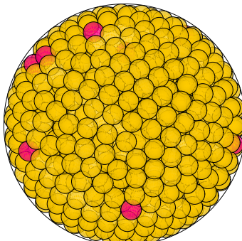
N = 995 995 spheres in a sphere
