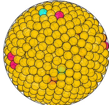
N = 993 993 spheres in a sphere
