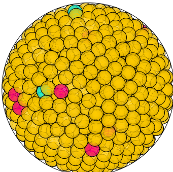
N = 994 994 spheres in a sphere
