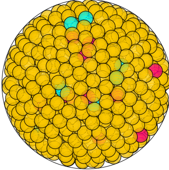
N = 961 961 spheres in a sphere
