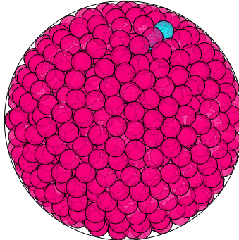
N = 965 965 spheres in a sphere
