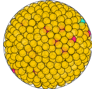
N = 966 966 spheres in a sphere
