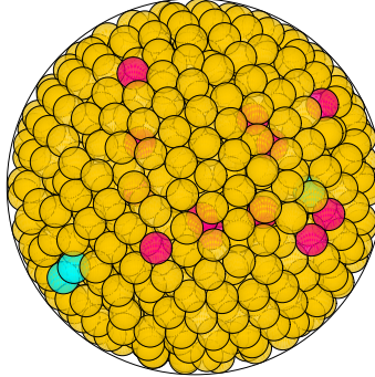
N = 962 962 spheres in a sphere
