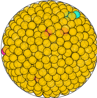
N = 964 964 spheres in a sphere
