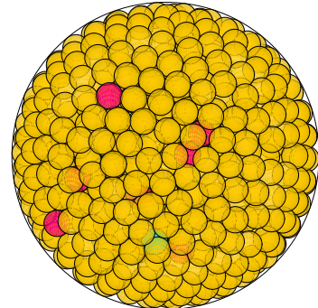
N = 972 972 spheres in a sphere
