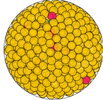
N = 963 963 spheres in a sphere
