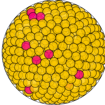
N = 968 968 spheres in a sphere
