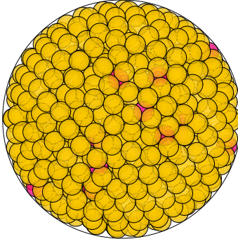
N = 967 967 spheres in a sphere
