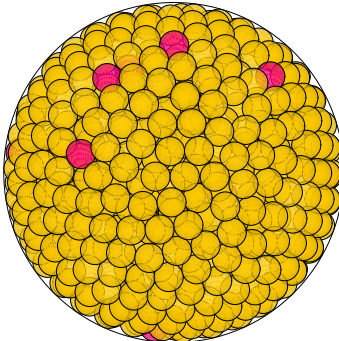
N = 970 970 spheres in a sphere
