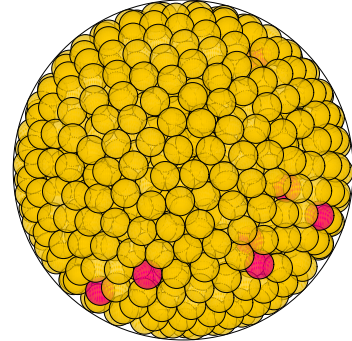
N = 969 969 spheres in a sphere
