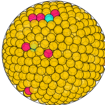
N = 971 971 spheres in a sphere
