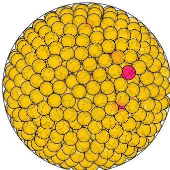
N = 959 959 spheres in a sphere
