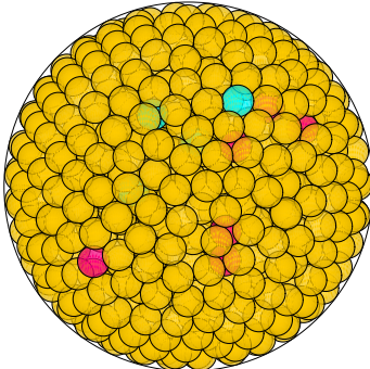
N = 955 955 spheres in a sphere
