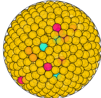
N = 957 957 spheres in a sphere
