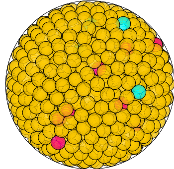
N = 954 954 spheres in a sphere
