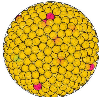
N = 960 960 spheres in a sphere
