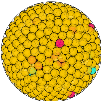
N = 958 958 spheres in a sphere
