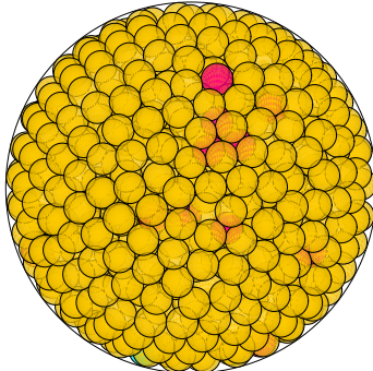
N = 956 956 spheres in a sphere
