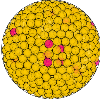
N = 950 950 spheres in a sphere
