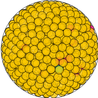
N = 952 952 spheres in a sphere
