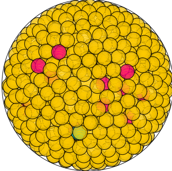
N = 949 949 spheres in a sphere
