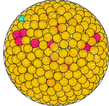
N = 951 951 spheres in a sphere
