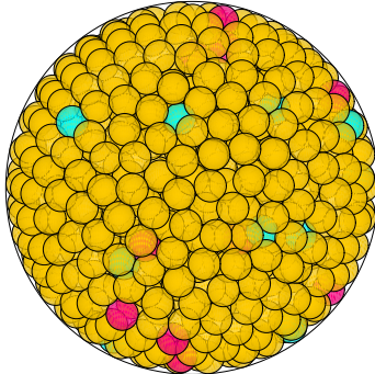
N = 953 953 spheres in a sphere
