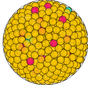
N = 939 939 spheres in a sphere
