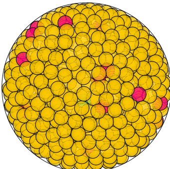
N = 946 946 spheres in a sphere
