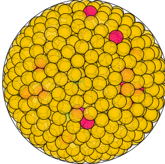
N = 938 938 spheres in a sphere
