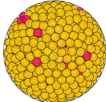
N = 945 945 spheres in a sphere
