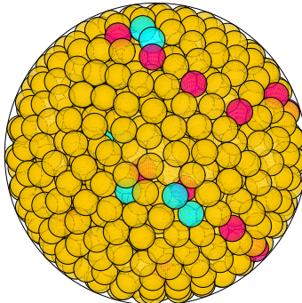
N = 941 941 spheres in a sphere
