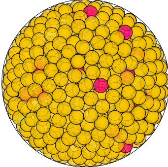
N = 937 937 spheres in a sphere
