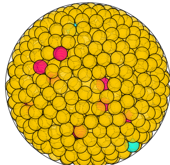
N = 948 948 spheres in a sphere
