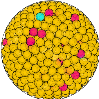
N = 943 943 spheres in a sphere
