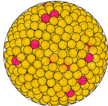
N = 942 942 spheres in a sphere
