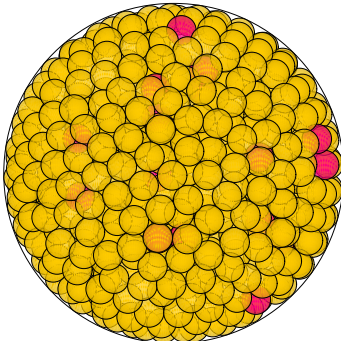
N = 940 940 spheres in a sphere
