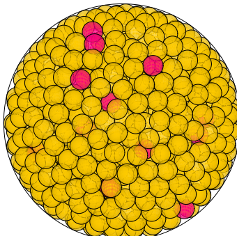
N = 947 947 spheres in a sphere
