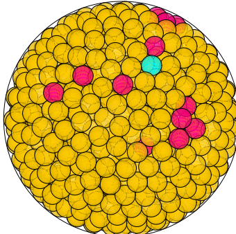
N = 944 944 spheres in a sphere
