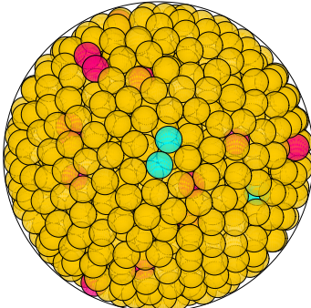
N = 931 931 spheres in a sphere
