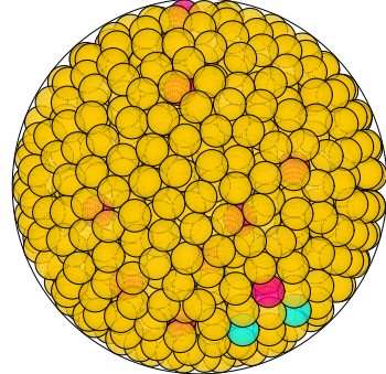
N = 927 927 spheres in a sphere
