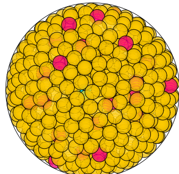
N = 936 936 spheres in a sphere
