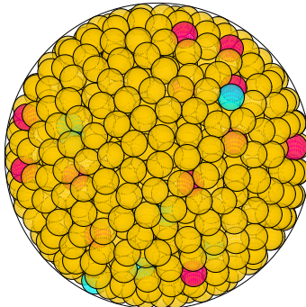
N = 929 929 spheres in a sphere
