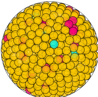
N = 934 934 spheres in a sphere
