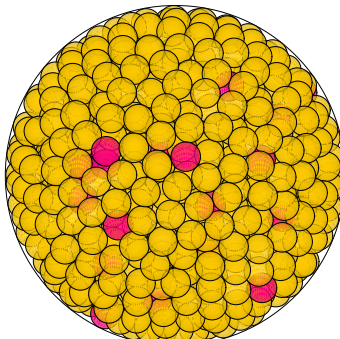
N = 935 935 spheres in a sphere
