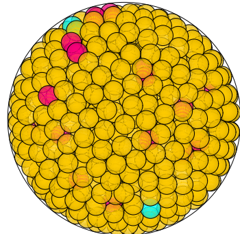
N = 930 930 spheres in a sphere
