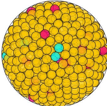
N = 932 932 spheres in a sphere
