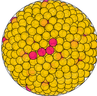
N = 926 926 spheres in a sphere
