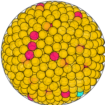
N = 928 928 spheres in a sphere
