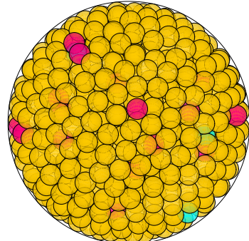
N = 933 933 spheres in a sphere
