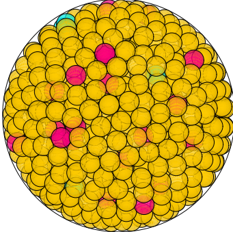
N = 925 925 spheres in a sphere
