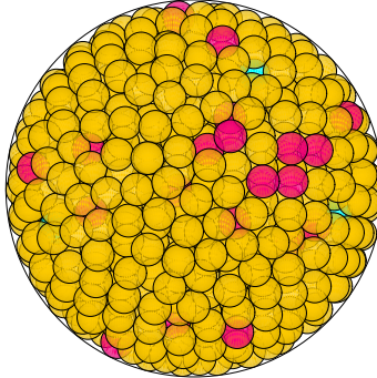
N = 920 920 spheres in a sphere
