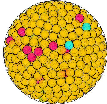
N = 918 918 spheres in a sphere
