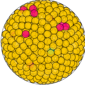
N = 913 913 spheres in a sphere
