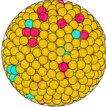
N = 914 914 spheres in a sphere
