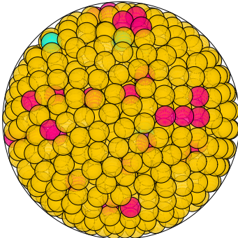
N = 922 922 spheres in a sphere
