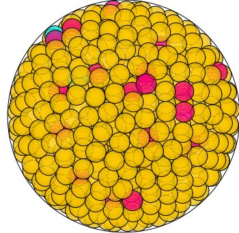
N = 921 921 spheres in a sphere
