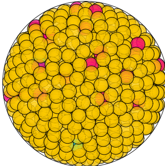
N = 923 923 spheres in a sphere
