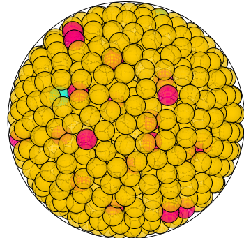
N = 924 924 spheres in a sphere
