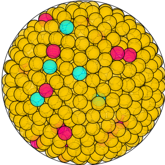
N = 916 916 spheres in a sphere
