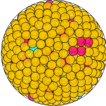
N = 919 919 spheres in a sphere
