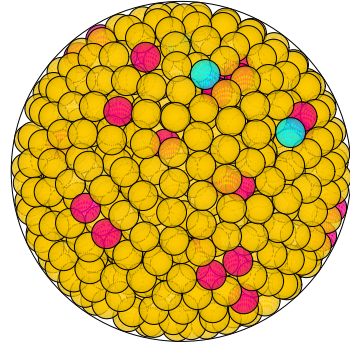
N = 906 906 spheres in a sphere
