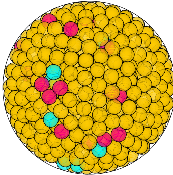
N = 908 908 spheres in a sphere
