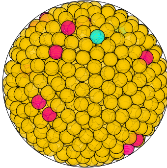
N = 905 905 spheres in a sphere
