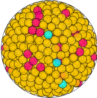
N = 904 904 spheres in a sphere
