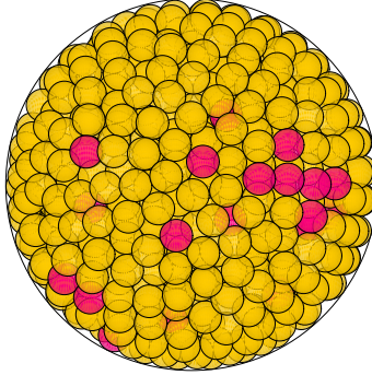
N = 902 902 spheres in a sphere
