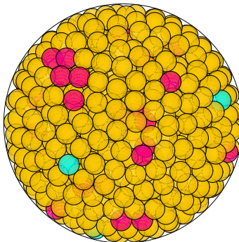
N = 911 911 spheres in a sphere
