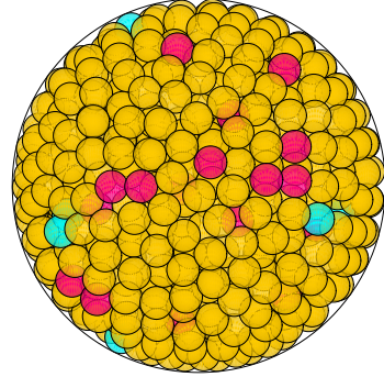
N = 903 903 spheres in a sphere
