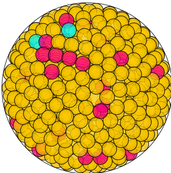
N = 910 910 spheres in a sphere
