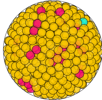
N = 909 909 spheres in a sphere
