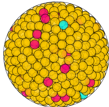
N = 912 912 spheres in a sphere
