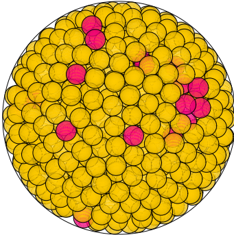
N = 907 907 spheres in a sphere
