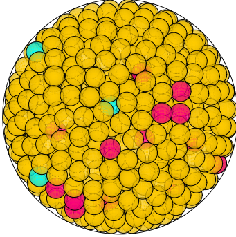
N = 901 901 spheres in a sphere
