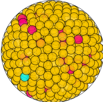
N = 892 892 spheres in a sphere
