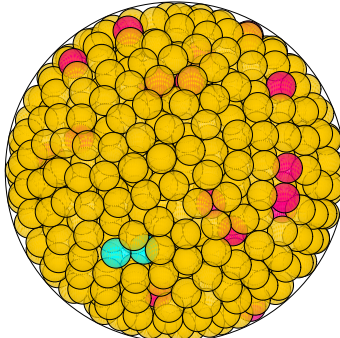
N = 896 896 spheres in a sphere
