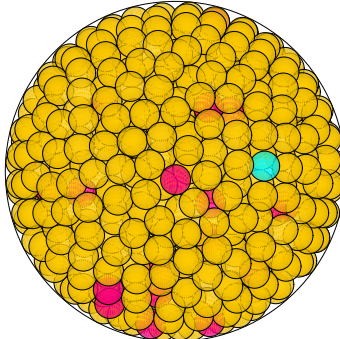
N = 893 893 spheres in a sphere
