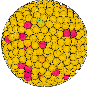
N = 890 890 spheres in a sphere
