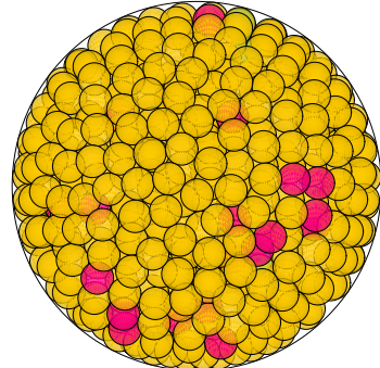
N = 894 894 spheres in a sphere
