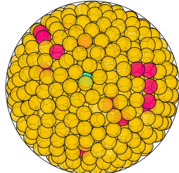
N = 897 897 spheres in a sphere
