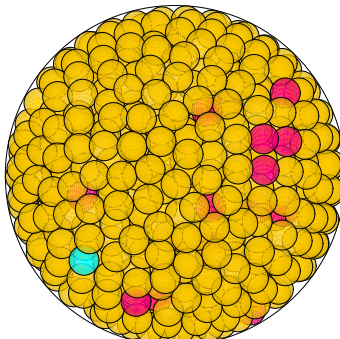
N = 899 899 spheres in a sphere
