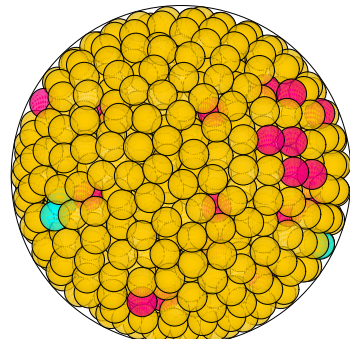
N = 900 900 spheres in a sphere
