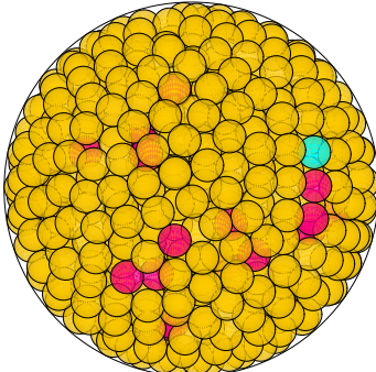
N = 895 895 spheres in a sphere
