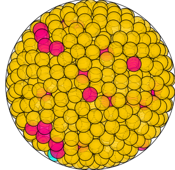
N = 891 891 spheres in a sphere
