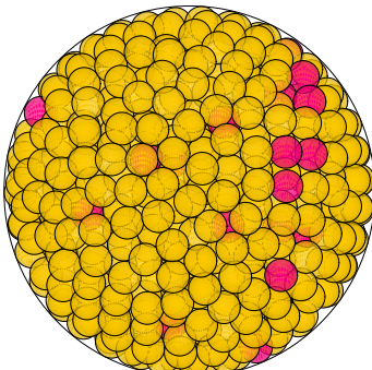
N = 898 898 spheres in a sphere
