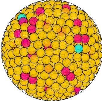
N = 889 889 spheres in a sphere
