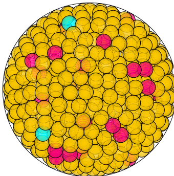
N = 887 887 spheres in a sphere
