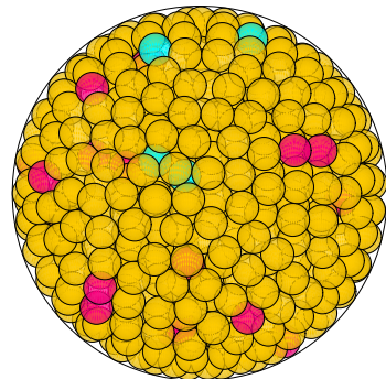
N = 888 888 spheres in a sphere
