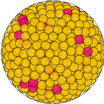
N = 883 883 spheres in a sphere
