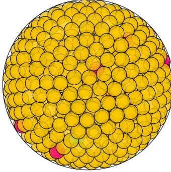
N = 878 878 spheres in a sphere
