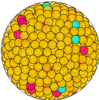
N = 886 886 spheres in a sphere
