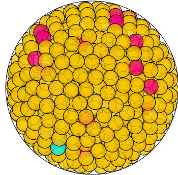
N = 885 885 spheres in a sphere
