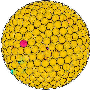
N = 880 880 spheres in a sphere
