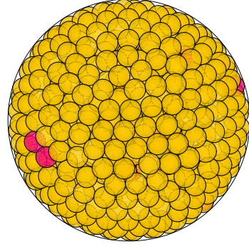
N = 879 879 spheres in a sphere
