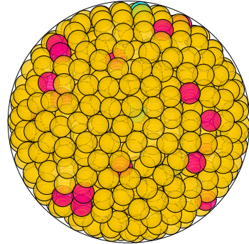
N = 882 882 spheres in a sphere
