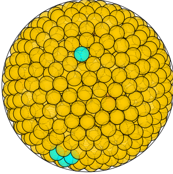
N = 877 877 spheres in a sphere
