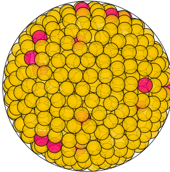
N = 884 884 spheres in a sphere
