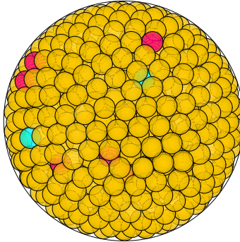
N = 881 881 spheres in a sphere
