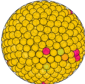
N = 872 872 spheres in a sphere
