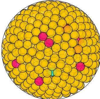
N = 869 869 spheres in a sphere
