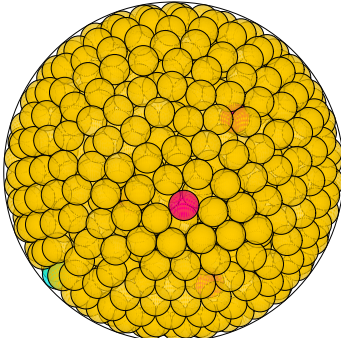
N = 871 871 spheres in a sphere
