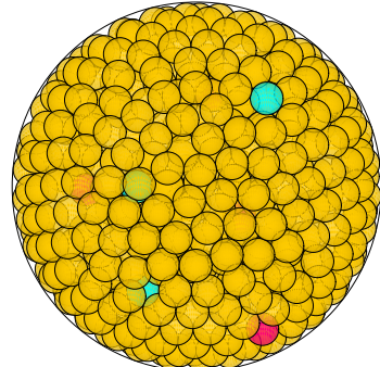
N = 873 873 spheres in a sphere
