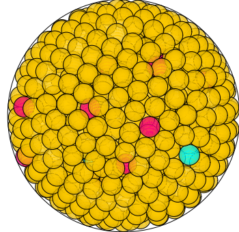
N = 867 867 spheres in a sphere
