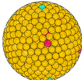
N = 876 876 spheres in a sphere
