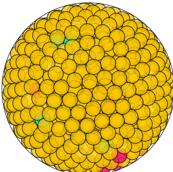
N = 874 874 spheres in a sphere
