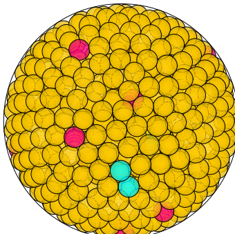
N = 875 875 spheres in a sphere
