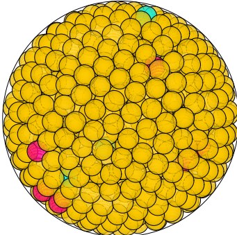
N = 868 868 spheres in a sphere
