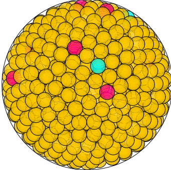
N = 865 865 spheres in a sphere
