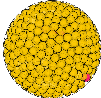
N = 870 870 spheres in a sphere
