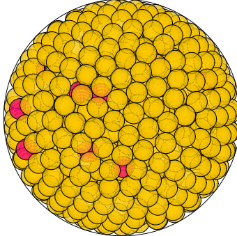
N = 866 866 spheres in a sphere
