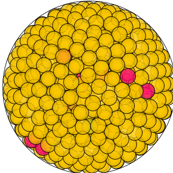
N = 860 860 spheres in a sphere
