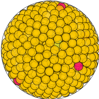
N = 862 862 spheres in a sphere
