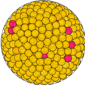
N = 856 856 spheres in a sphere
