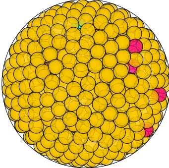
N = 853 853 spheres in a sphere
