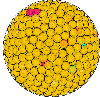
N = 855 855 spheres in a sphere
