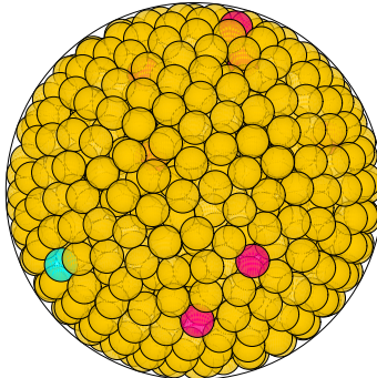
N = 863 863 spheres in a sphere
