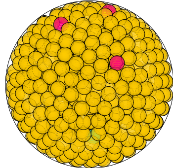
N = 858 858 spheres in a sphere
