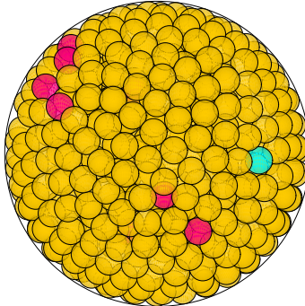
N = 857 857 spheres in a sphere
