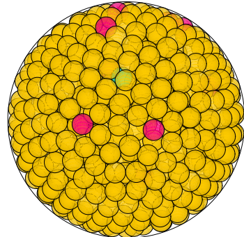
N = 864 864 spheres in a sphere
