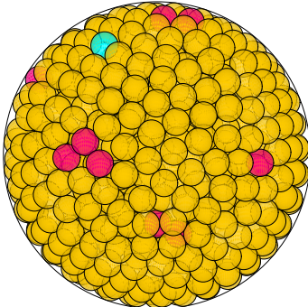
N = 859 859 spheres in a sphere
