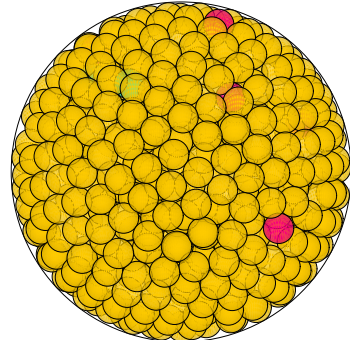
N = 861 861 spheres in a sphere
