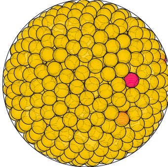
N = 854 854 spheres in a sphere
