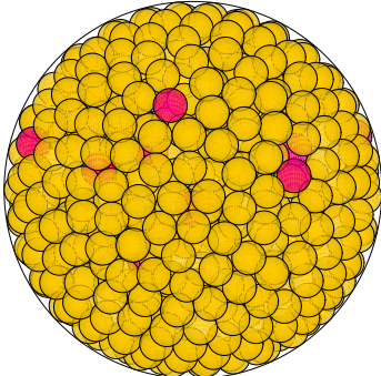
N = 844 844 spheres in a sphere
