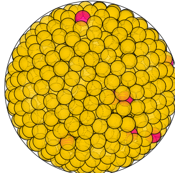
N = 849 849 spheres in a sphere
