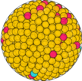
N = 841 841 spheres in a sphere
