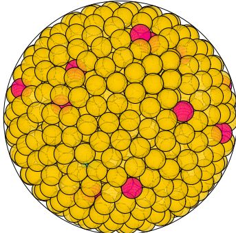
N = 845 845 spheres in a sphere
