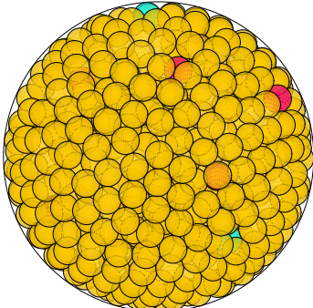
N = 847 847 spheres in a sphere
