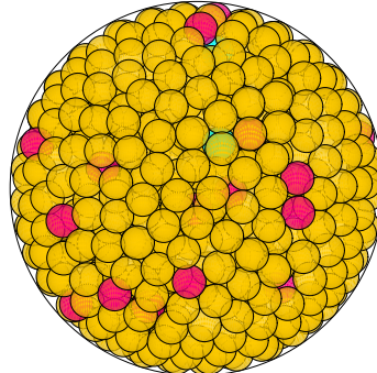
N = 846 846 spheres in a sphere
