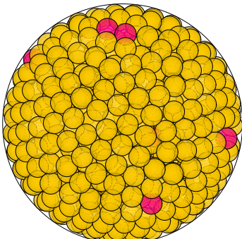
N = 850 850 spheres in a sphere
