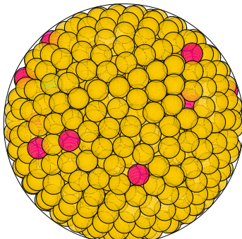
N = 851 851 spheres in a sphere
