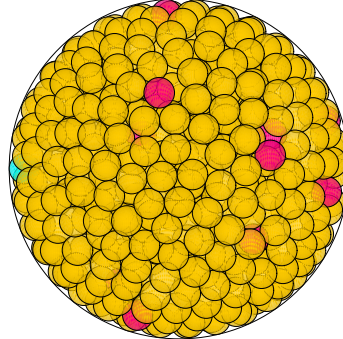
N = 843 843 spheres in a sphere
