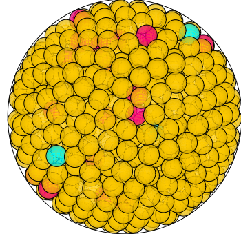
N = 831 831 spheres in a sphere
