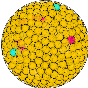
N = 833 833 spheres in a sphere
