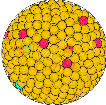
N = 830 830 spheres in a sphere
