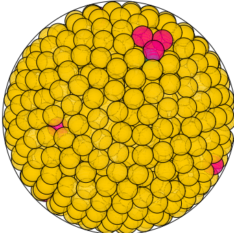
N = 832 832 spheres in a sphere
