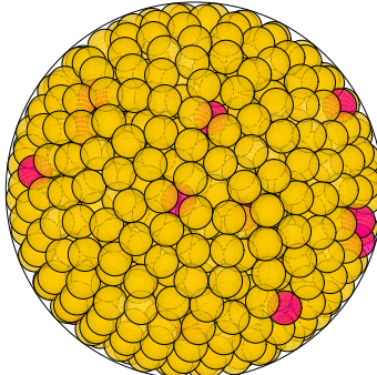
N = 836 836 spheres in a sphere
