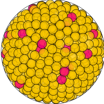
N = 829 829 spheres in a sphere
