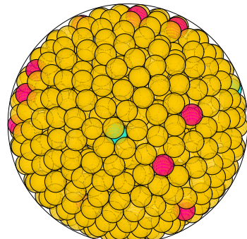
N = 840 840 spheres in a sphere
