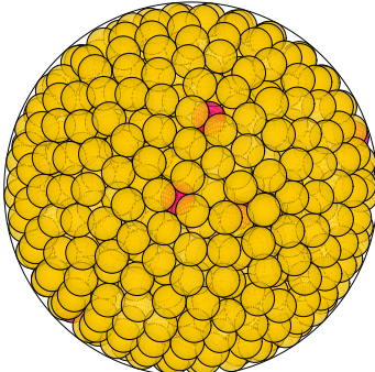
N = 835 835 spheres in a sphere
