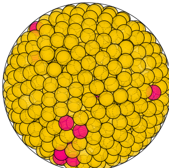
N = 839 839 spheres in a sphere
