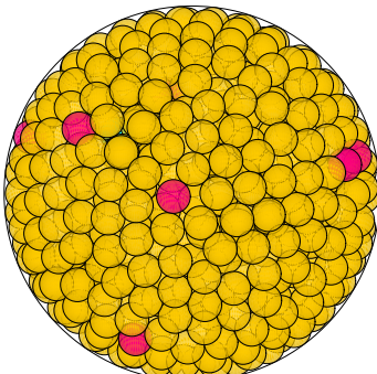
N = 838 838 spheres in a sphere
