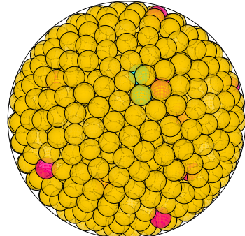
N = 837 837 spheres in a sphere
