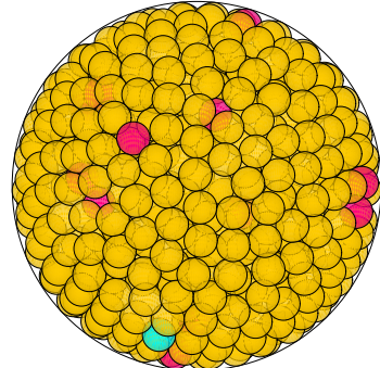
N = 834 834 spheres in a sphere
