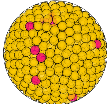
N = 825 825 spheres in a sphere
