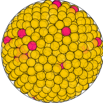
N = 817 817 spheres in a sphere
