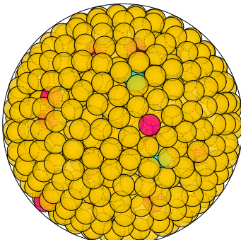
N = 826 826 spheres in a sphere
