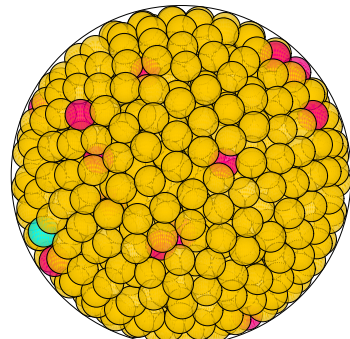
N = 828 828 spheres in a sphere
