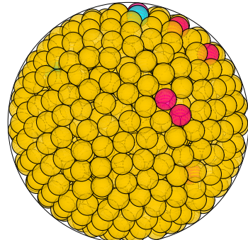
N = 822 822 spheres in a sphere
