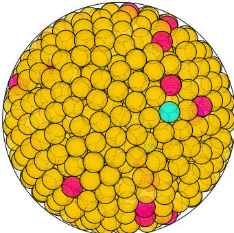
N = 820 820 spheres in a sphere
