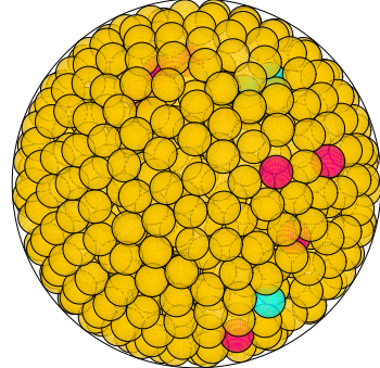
N = 819 819 spheres in a sphere
