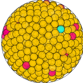
N = 818 818 spheres in a sphere
