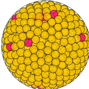
N = 824 824 spheres in a sphere
