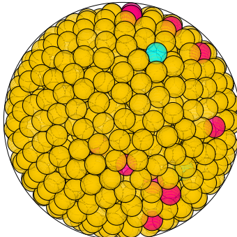
N = 821 821 spheres in a sphere
