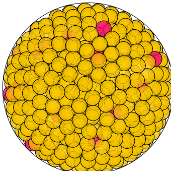
N = 827 827 spheres in a sphere
