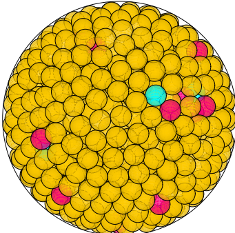
N = 823 823 spheres in a sphere
