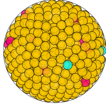
N = 807 807 spheres in a sphere
