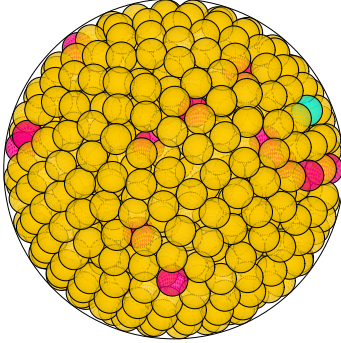
N = 805 805 spheres in a sphere
