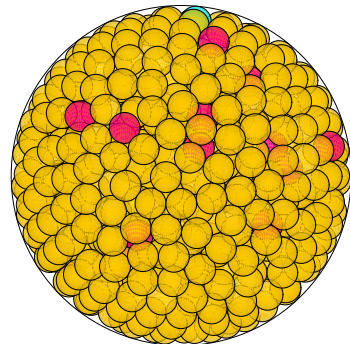
N = 816 816 spheres in a sphere
