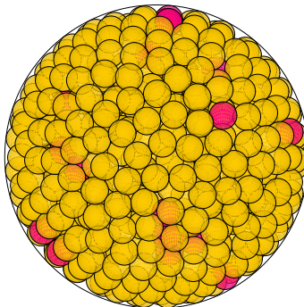
N = 815 815 spheres in a sphere
