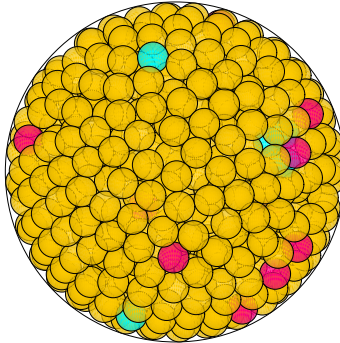
N = 812 812 spheres in a sphere
