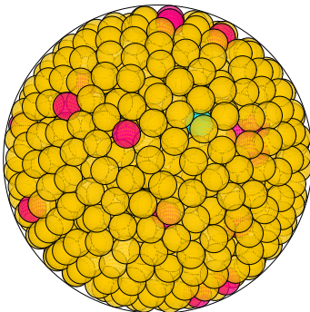
N = 814 814 spheres in a sphere
