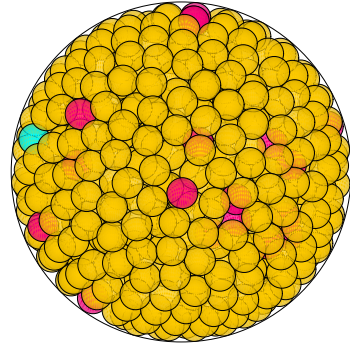
N = 813 813 spheres in a sphere
