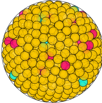
N = 809 809 spheres in a sphere
