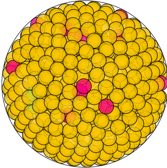
N = 808 808 spheres in a sphere
