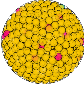
N = 806 806 spheres in a sphere
