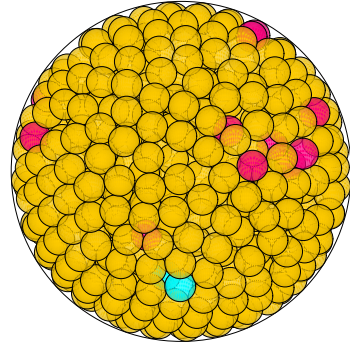
N = 810 810 spheres in a sphere
