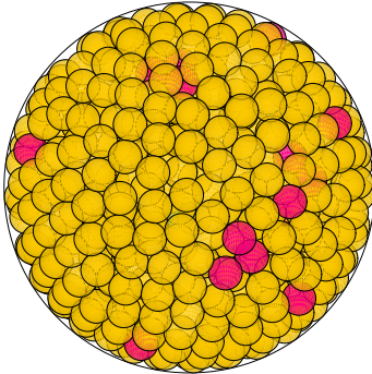
N = 811 811 spheres in a sphere
