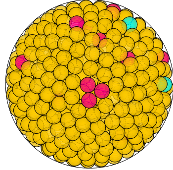
N = 786 786 spheres in a sphere
