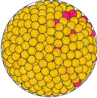
N = 787 787 spheres in a sphere
