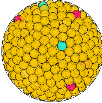
N = 785 785 spheres in a sphere
