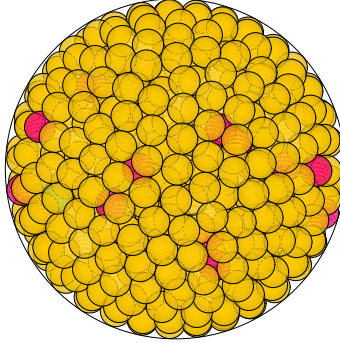
N = 782 782 spheres in a sphere
