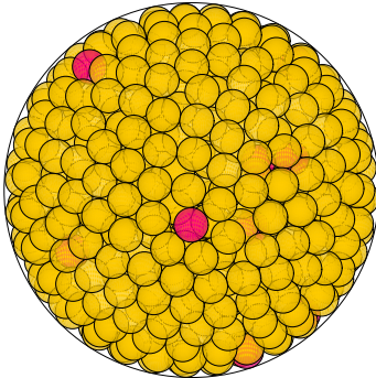
N = 790 790 spheres in a sphere
