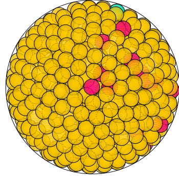
N = 789 789 spheres in a sphere
