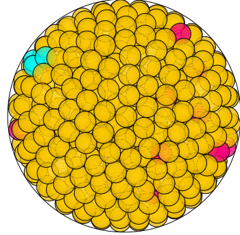
N = 783 783 spheres in a sphere
