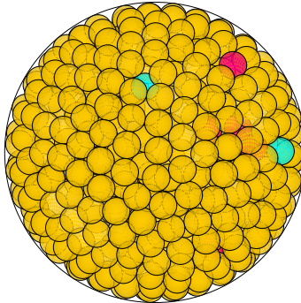
N = 791 791 spheres in a sphere
