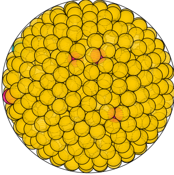
N = 781 781 spheres in a sphere
