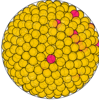
N = 788 788 spheres in a sphere
