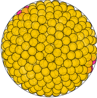
N = 784 784 spheres in a sphere
