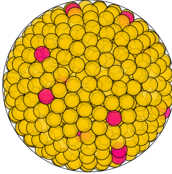
N = 776 776 spheres in a sphere
