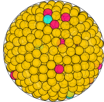
N = 774 774 spheres in a sphere
