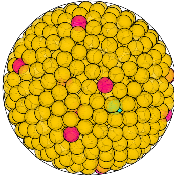
N = 773 773 spheres in a sphere
