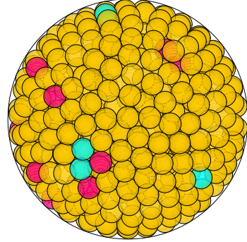
N = 771 771 spheres in a sphere
