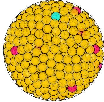
N = 777 777 spheres in a sphere
