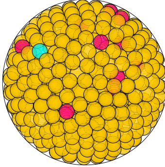
N = 770 770 spheres in a sphere
