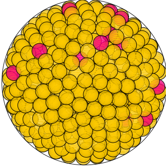
N = 769 769 spheres in a sphere
