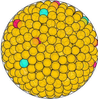
N = 772 772 spheres in a sphere
