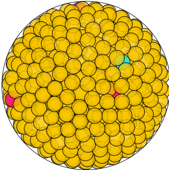
N = 778 778 spheres in a sphere
