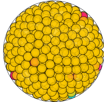
N = 780 780 spheres in a sphere
