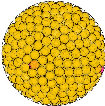
N = 779 779 spheres in a sphere
