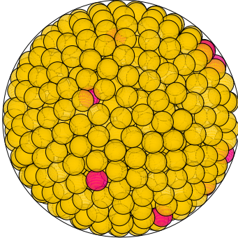
N = 775 775 spheres in a sphere
