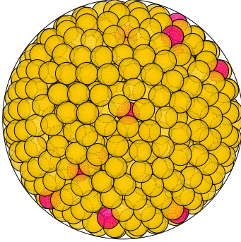
N = 757 757 spheres in a sphere
