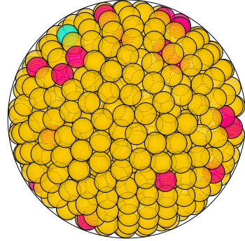
N = 765 765 spheres in a sphere
