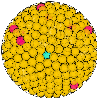
N = 767 767 spheres in a sphere
