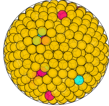
N = 759 759 spheres in a sphere
