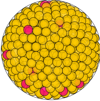
N = 763 763 spheres in a sphere
