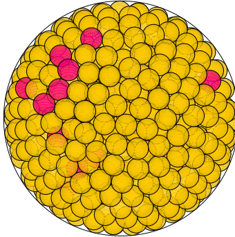
N = 761 761 spheres in a sphere
