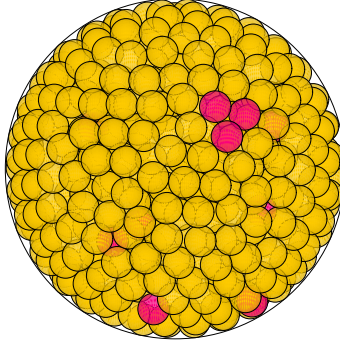
N = 758 758 spheres in a sphere
