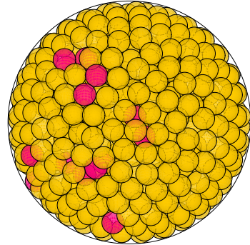
N = 762 762 spheres in a sphere
