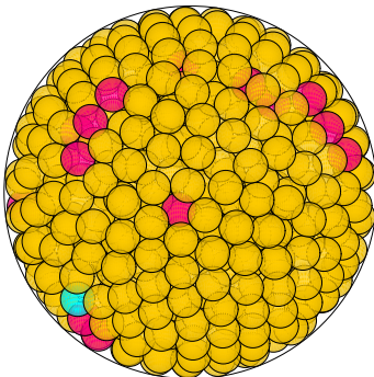
N = 766 766 spheres in a sphere
