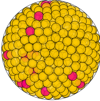
N = 764 764 spheres in a sphere
