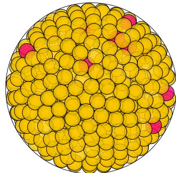
N = 768 768 spheres in a sphere
