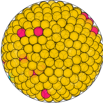
N = 760 760 spheres in a sphere
