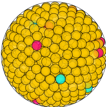
N = 754 754 spheres in a sphere
