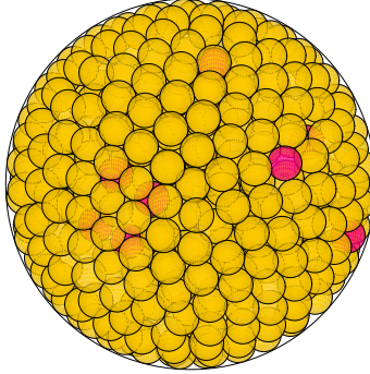
N = 746 746 spheres in a sphere
