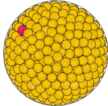
N = 753 753 spheres in a sphere
