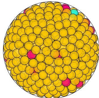
N = 756 756 spheres in a sphere
