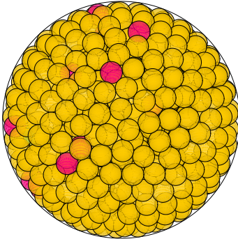
N = 751 751 spheres in a sphere
