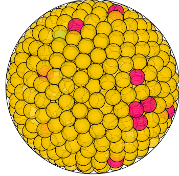
N = 747 747 spheres in a sphere
