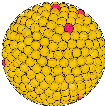
N = 755 755 spheres in a sphere
