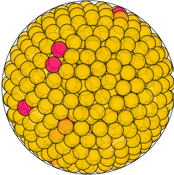
N = 748 748 spheres in a sphere
