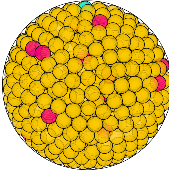
N = 752 752 spheres in a sphere
