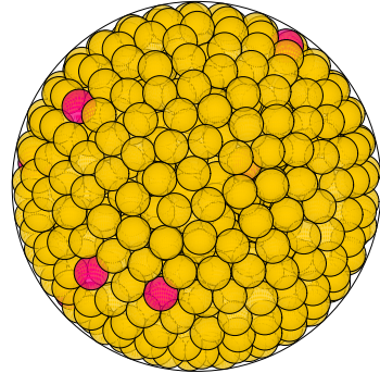
N = 750 750 spheres in a sphere
