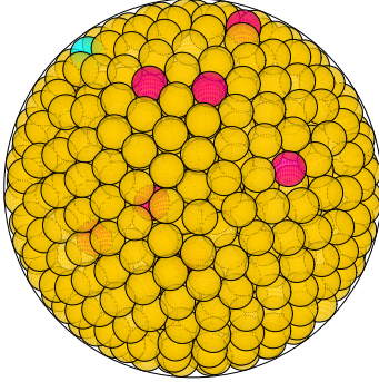
N = 745 745 spheres in a sphere
