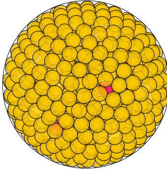
N = 749 749 spheres in a sphere
