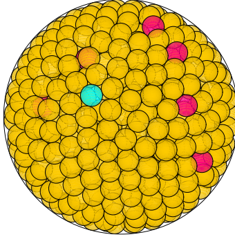
N = 734 734 spheres in a sphere
