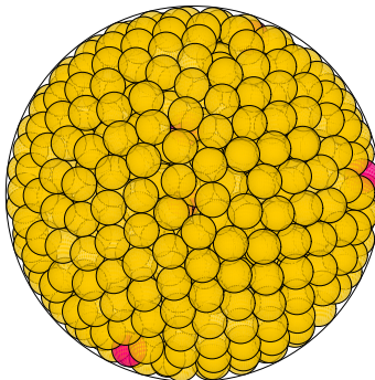
N = 743 743 spheres in a sphere
