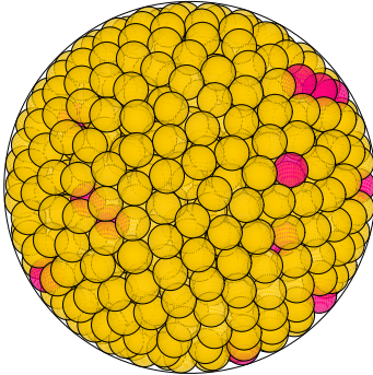
N = 736 736 spheres in a sphere
