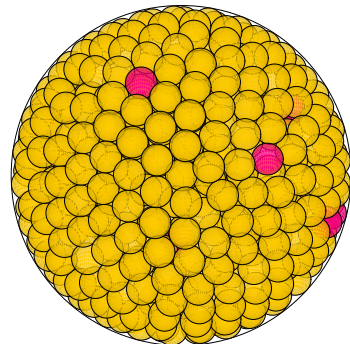
N = 744 744 spheres in a sphere
