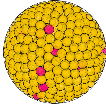
N = 738 738 spheres in a sphere
