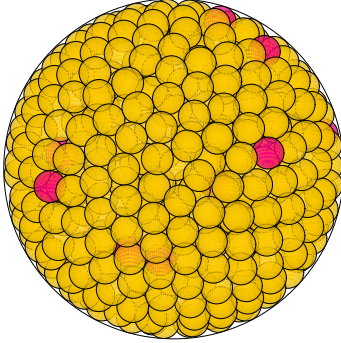
N = 733 733 spheres in a sphere
