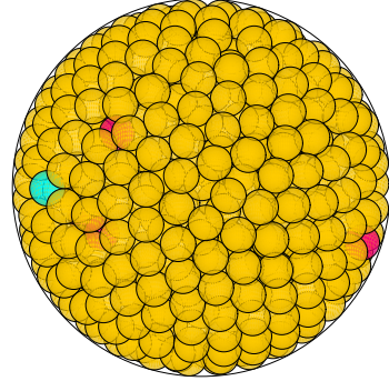
N = 735 735 spheres in a sphere
