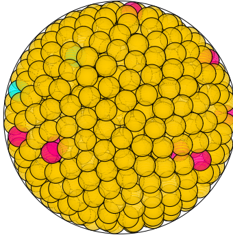
N = 737 737 spheres in a sphere
