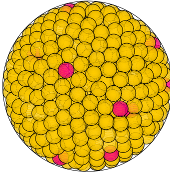
N = 740 740 spheres in a sphere
