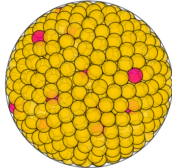
N = 741 741 spheres in a sphere
