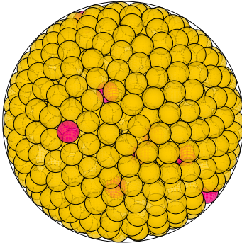
N = 739 739 spheres in a sphere
