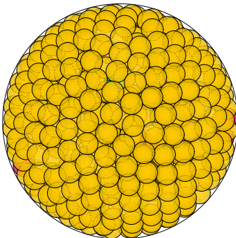
N = 742 742 spheres in a sphere
