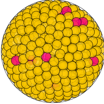
N = 721 721 spheres in a sphere
