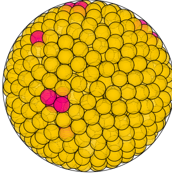
N = 728 728 spheres in a sphere
