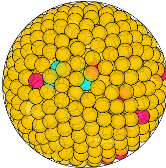
N = 731 731 spheres in a sphere
