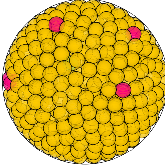
N = 722 722 spheres in a sphere
