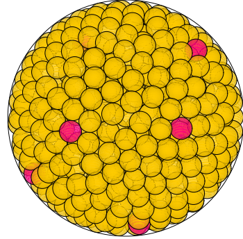
N = 729 729 spheres in a sphere
