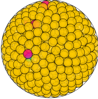
N = 727 727 spheres in a sphere
