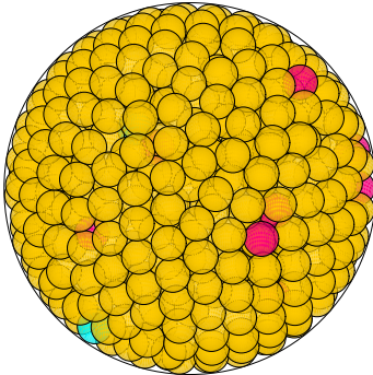
N = 730 730 spheres in a sphere
