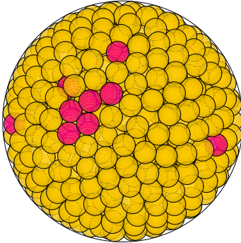
N = 724 724 spheres in a sphere
