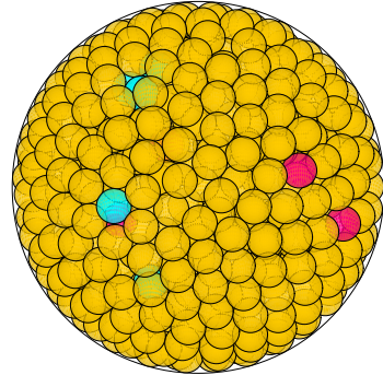
N = 726 726 spheres in a sphere
