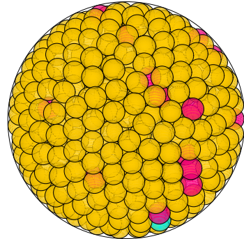
N = 732 732 spheres in a sphere
