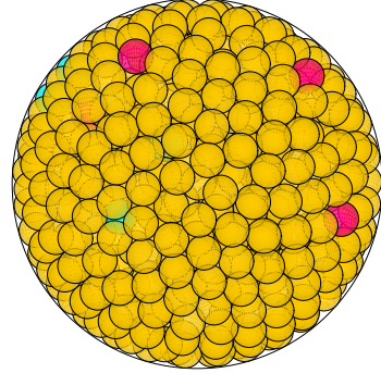
N = 723 723 spheres in a sphere
