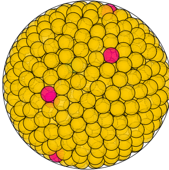
N = 725 725 spheres in a sphere
