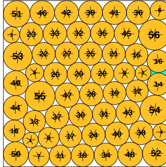
N = 56 56 circles in a square
