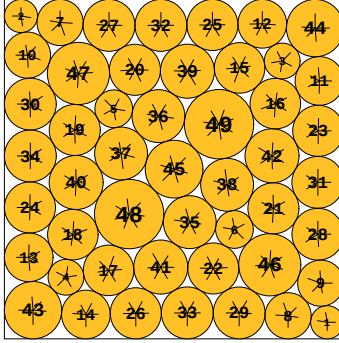
N = 49 49 circles in a square
