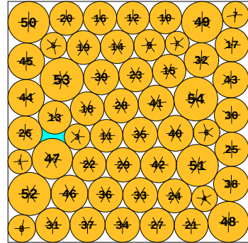
N = 54 54 circles in a square
