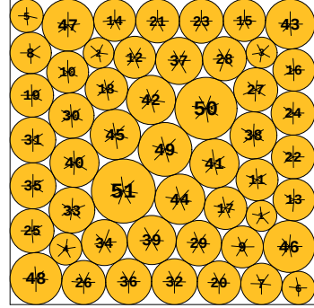
N = 51 51 circles in a square
