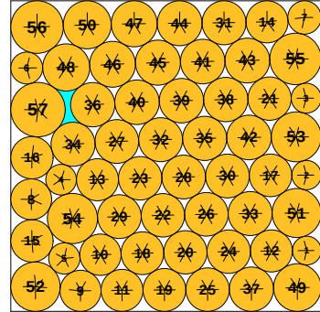
N = 57 57 circles in a square
