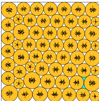
N = 58 58 circles in a square
