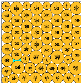
N = 59 59 circles in a square
