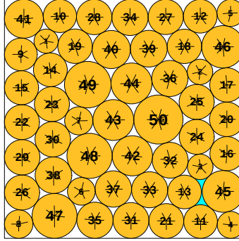
N = 50 50 circles in a square
