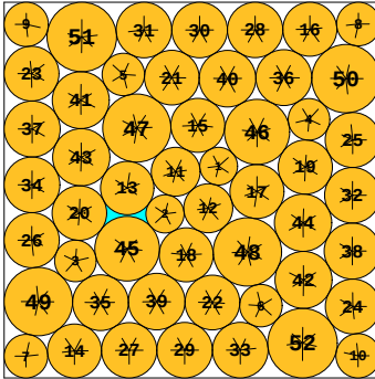
N = 52 52 circles in a square
