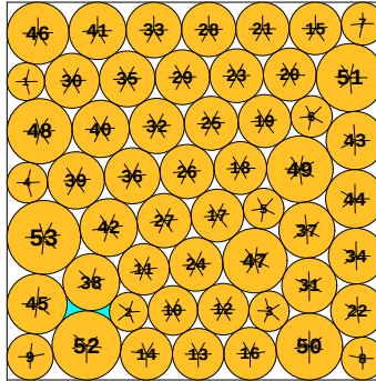
N = 53 53 circles in a square
