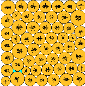
N = 55 55 circles in a square
