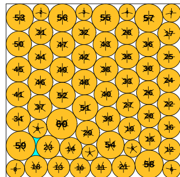
N = 60 60 circles in a square
