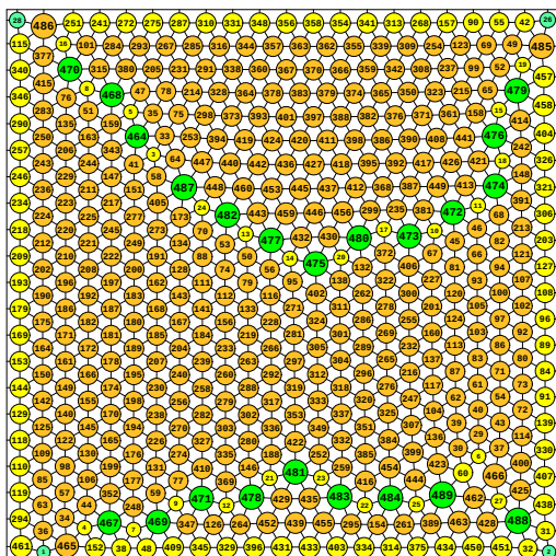
N = 489 489 circles in a square
