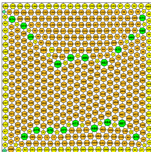
N = 488 488 circles in a square
