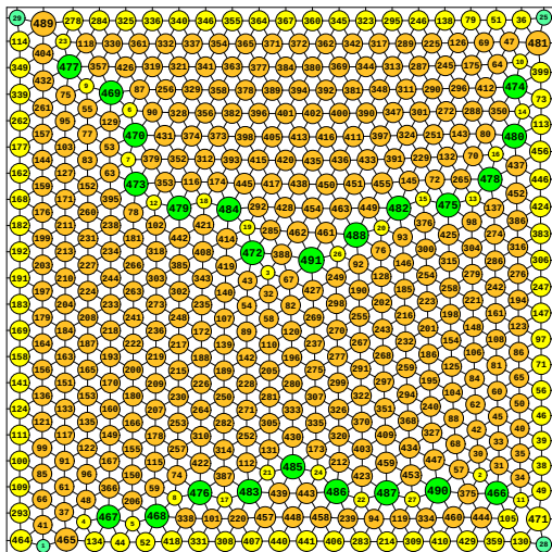
N = 491 491 circles in a square
