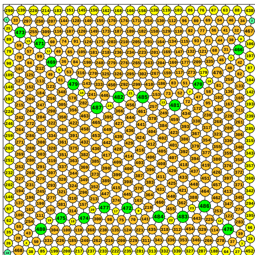
N = 487 487 circles in a square
