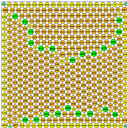
N = 492 492 circles in a square
