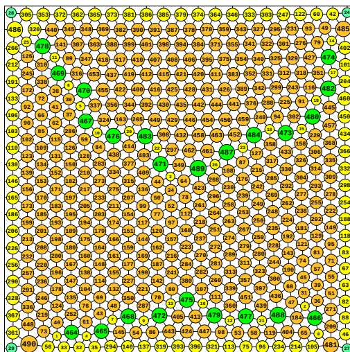
N = 490 490 circles in a square
