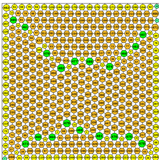
N = 482 482 circles in a square
