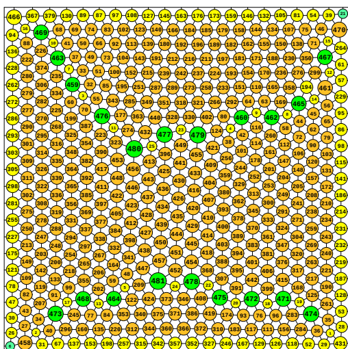
N = 481 481 circles in a square
