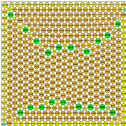
N = 486 486 circles in a square
