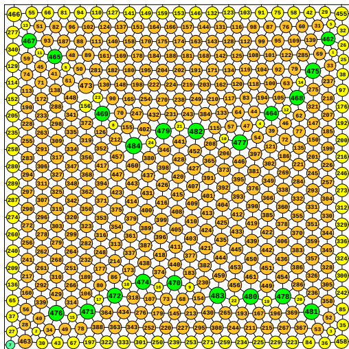
N = 484 484 circles in a square
