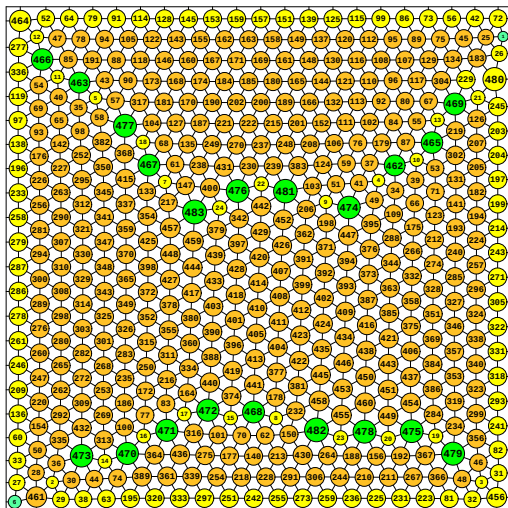
N = 483 483 circles in a square
