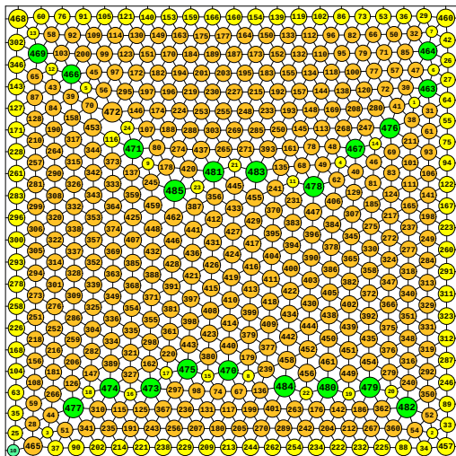
N = 485 485 circles in a square
