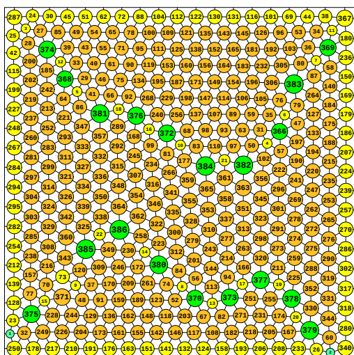
N = 386 386 circles in a square
