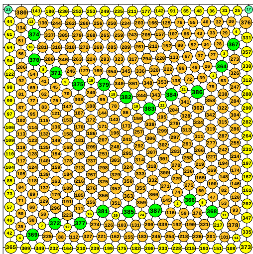
N = 387 387 circles in a square
