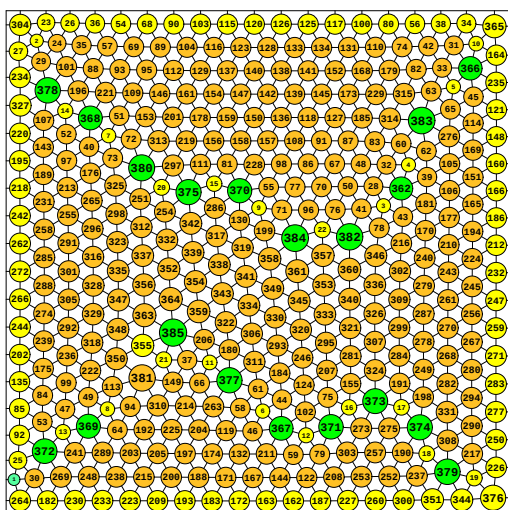
N = 385 385 circles in a square
