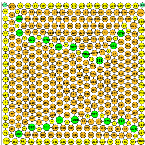
N = 389 389 circles in a square
