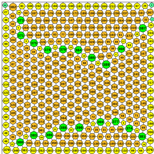
N = 390 390 circles in a square
