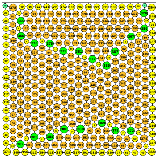
N = 388 388 circles in a square
