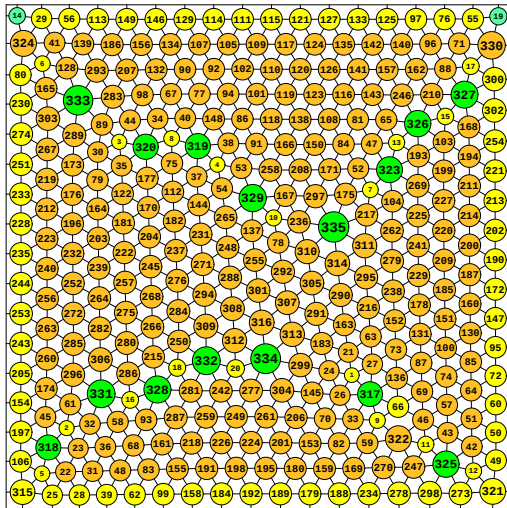
N = 335 335 circles in a square
