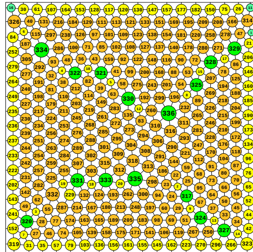
N = 336 336 circles in a square
