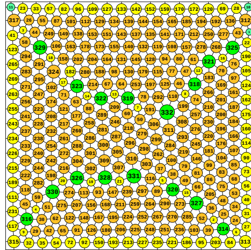
N = 332 332 circles in a square
