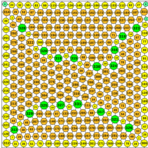
N = 331 331 circles in a square
