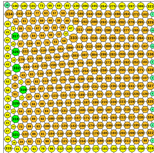
N = 334 334 circles in a square
