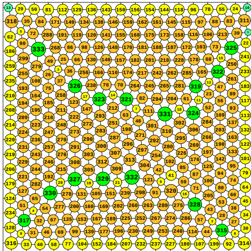
N = 333 333 circles in a square
