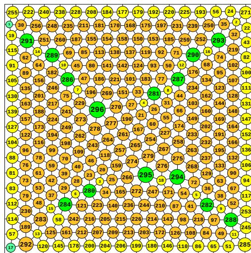
N = 296 296 circles in a square
