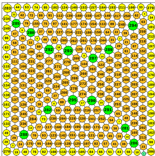
N = 295 295 circles in a square
