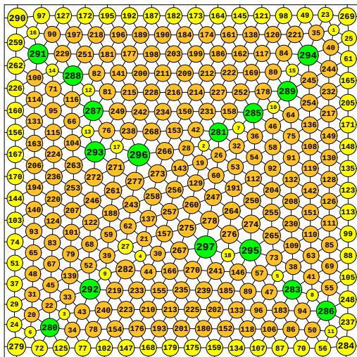
N = 297 297 circles in a square
