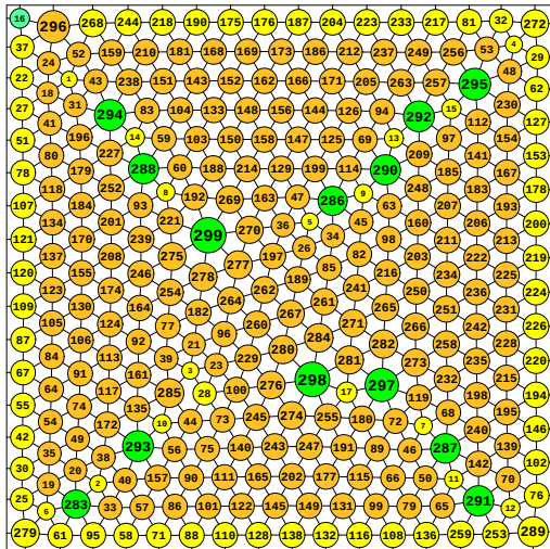
N = 299 299 circles in a square
