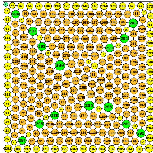
N = 300 300 circles in a square
