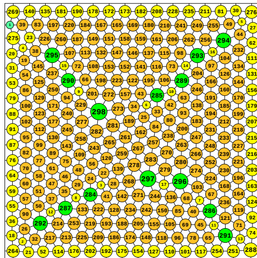
N = 298 298 circles in a square
