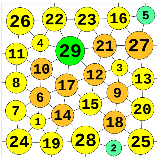
N = 29 29 circles in a square
