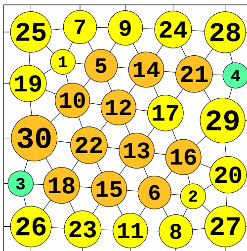
N = 30 30 circles in a square
