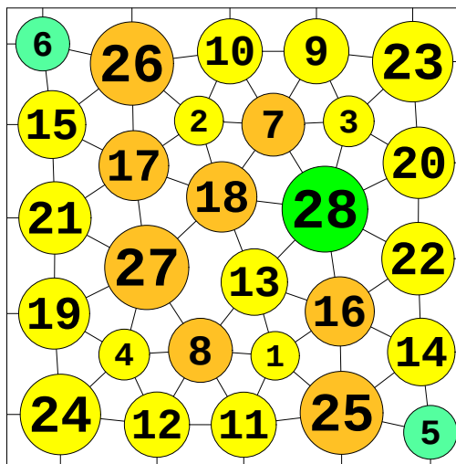
N = 28 28 circles in a square
