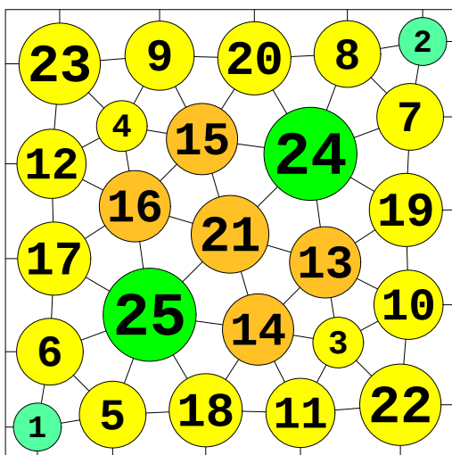
N = 25 25 circles in a square
