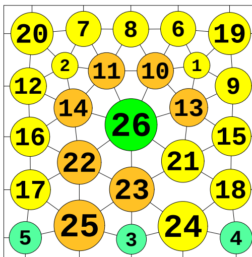
N = 26 26 circles in a square
