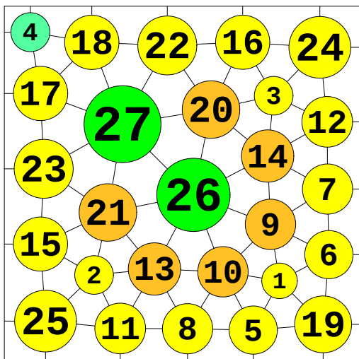
N = 27 27 circles in a square
