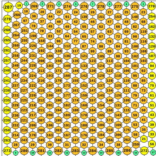
N = 287 287 circles in a square
