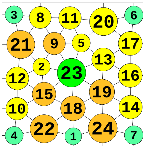
N = 24 24 circles in a square
