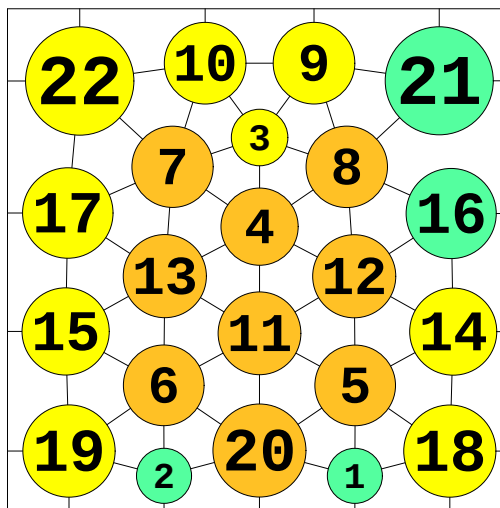
N = 22 22 circles in a square
