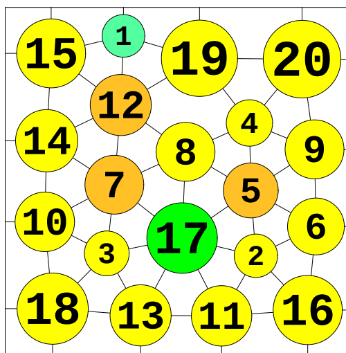
N = 20 20 circles in a square
