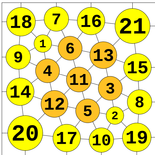
N = 21 21 circles in a square
