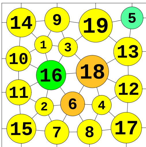
N = 19 19 circles in a square
