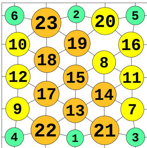
N = 23 23 circles in a square
