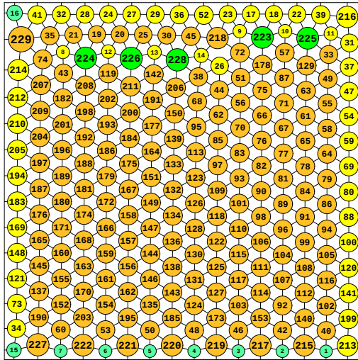
N = 229 229 circles in a square
