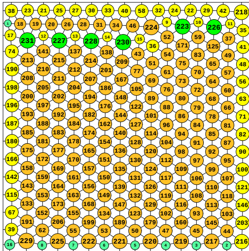
N = 231 231 circles in a square
