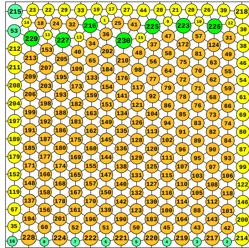
N = 230 230 circles in a square
