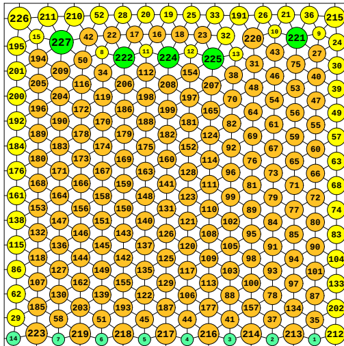
N = 227 227 circles in a square
