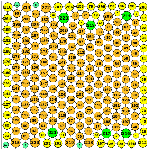
N = 223 223 circles in a square
