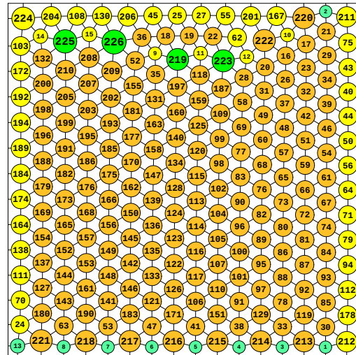
N = 226 226 circles in a square
