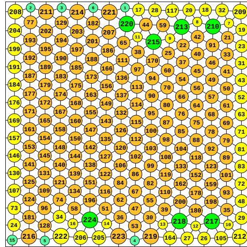
N = 224 224 circles in a square
