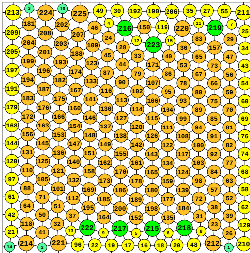
N = 225 225 circles in a square
