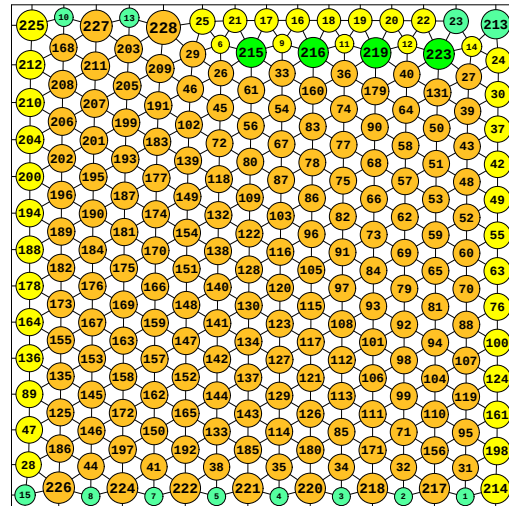
N = 228 228 circles in a square
