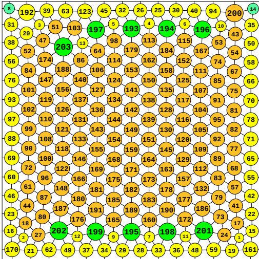
N = 203 203 circles in a square
