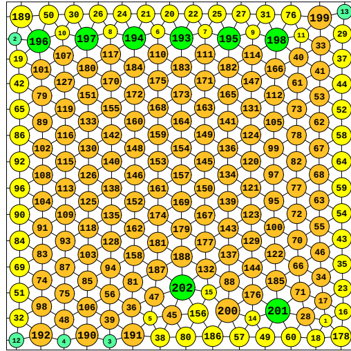
N = 202 202 circles in a square
