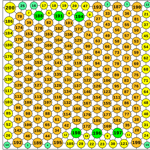
N = 200 200 circles in a square
