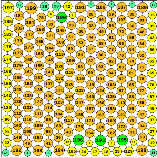
N = 199 199 circles in a square
