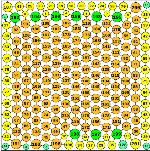
N = 201 201 circles in a square
