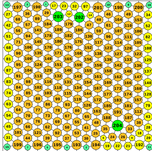
N = 204 204 circles in a square
