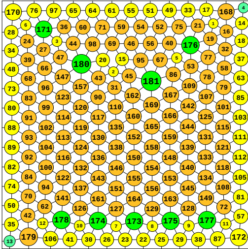
N = 181 181 circles in a square
