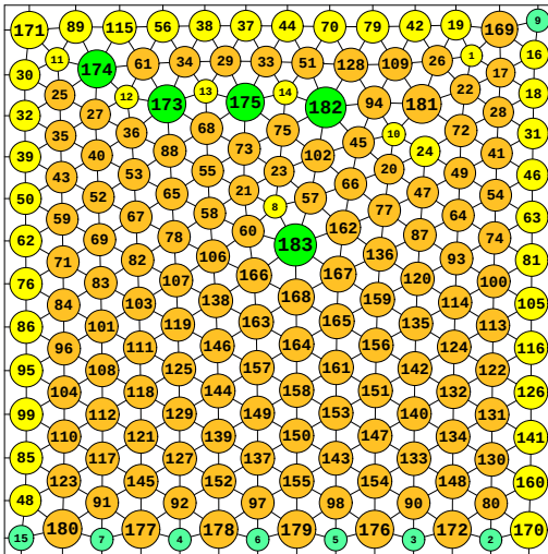
N = 183 183 circles in a square
