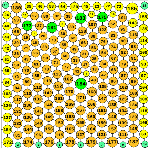
N = 185 185 circles in a square
