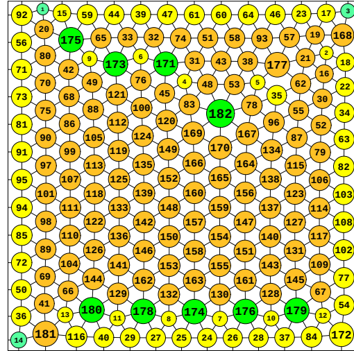
N = 182 182 circles in a square
