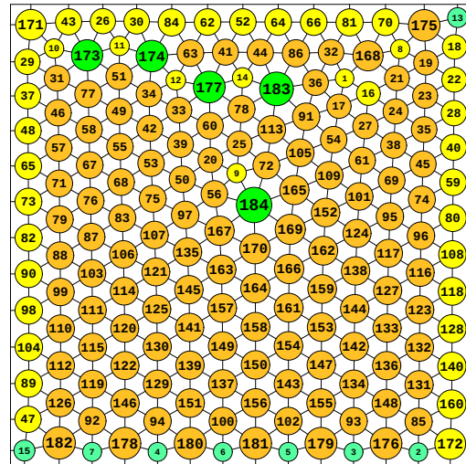
N = 184 184 circles in a square
