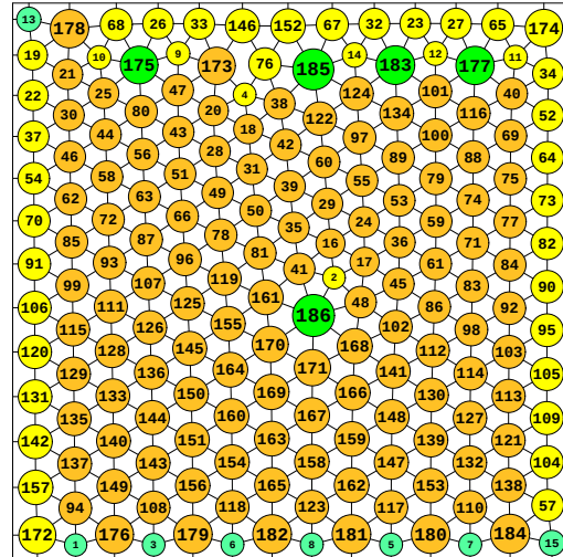
N = 186 186 circles in a square
