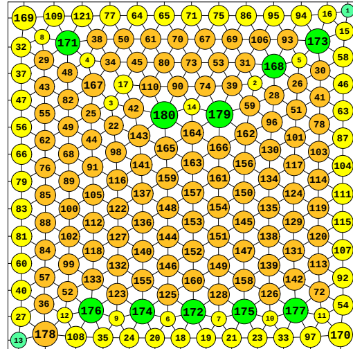
N = 180 180 circles in a square
