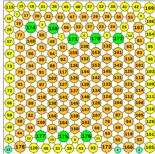
N = 178 178 circles in a square
