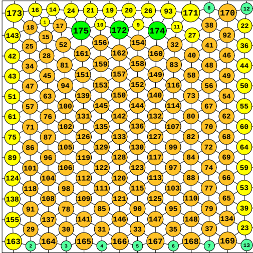
N = 175 175 circles in a square
