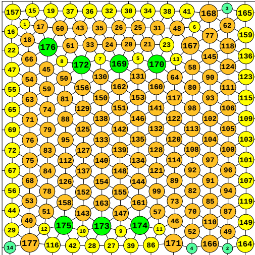
N = 177 177 circles in a square
