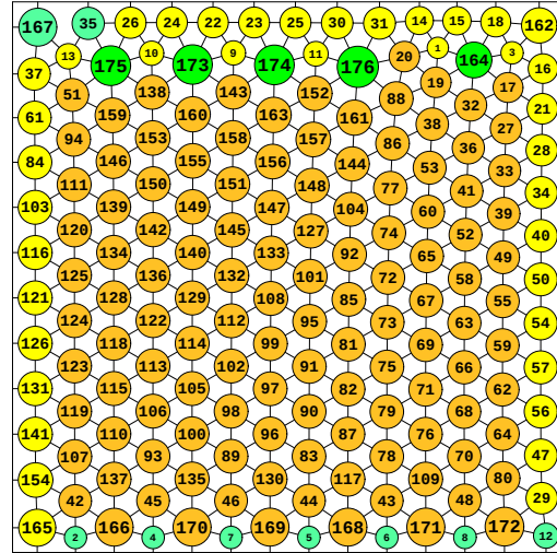
N = 176 176 circles in a square
