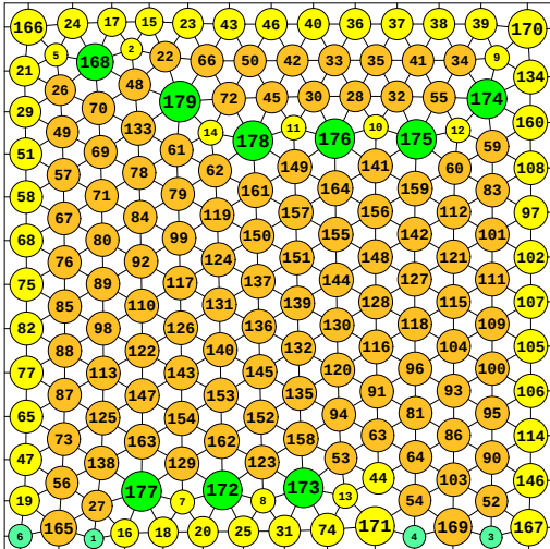
N = 179 179 circles in a square
