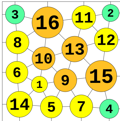
N = 16 16 circles in a square
