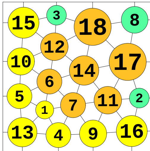
N = 18 18 circles in a square
