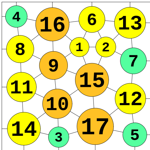
N = 17 17 circles in a square
