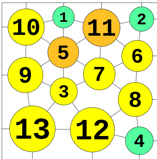
N = 13 13 circles in a square
