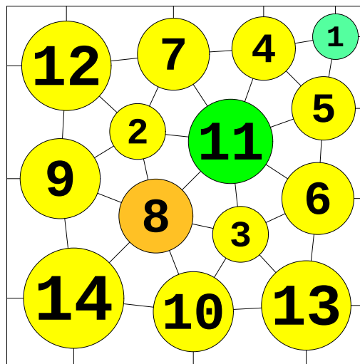
N = 14 14 circles in a square
