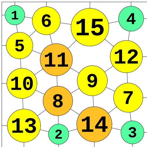
N = 15 15 circles in a square
