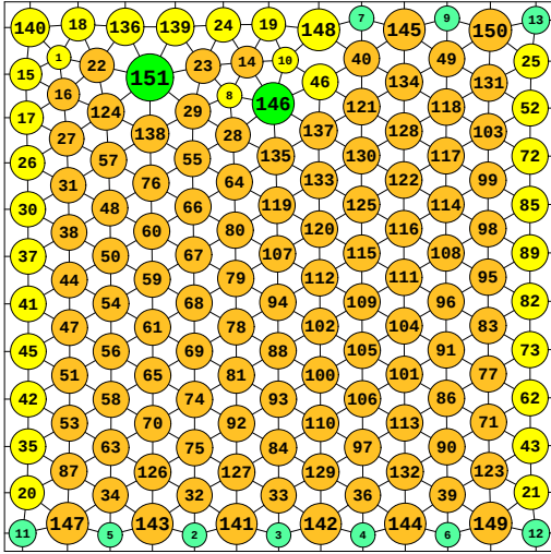
N = 151 151 circles in a square
