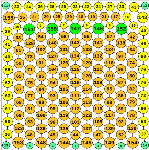
N = 155 155 circles in a square
