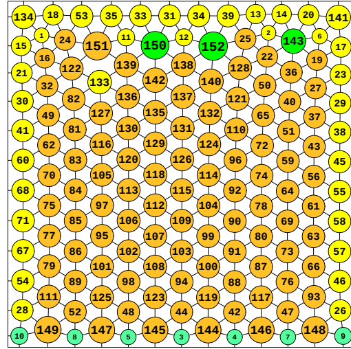
N = 152 152 circles in a square
