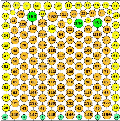
N = 153 153 circles in a square
