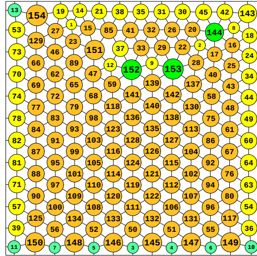
N = 154 154 circles in a square
