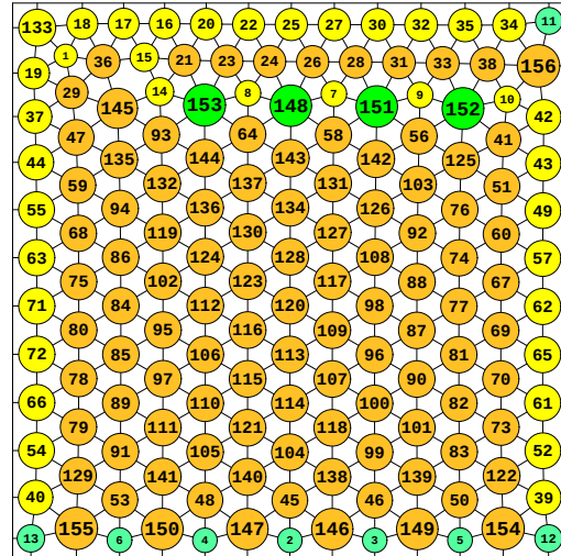
N = 156 156 circles in a square
