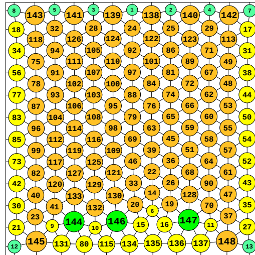
N = 148 148 circles in a square
