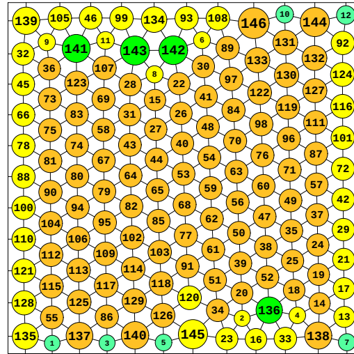
N = 146 146 circles in a square
