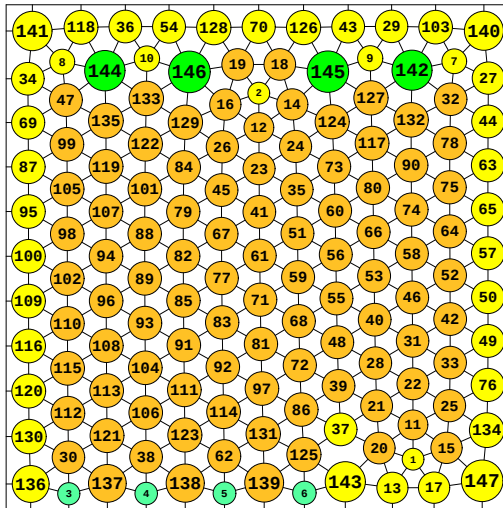
N = 147 147 circles in a square
