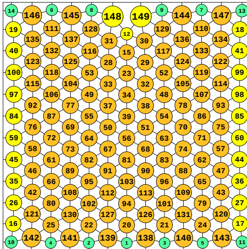
N = 149 149 circles in a square
