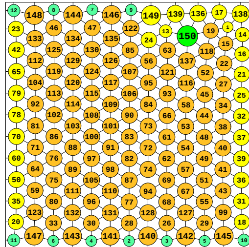
N = 150 150 circles in a square
