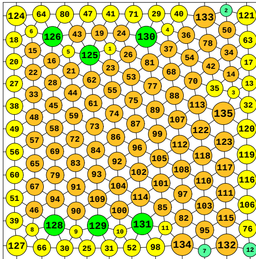
N = 135 135 circles in a square
