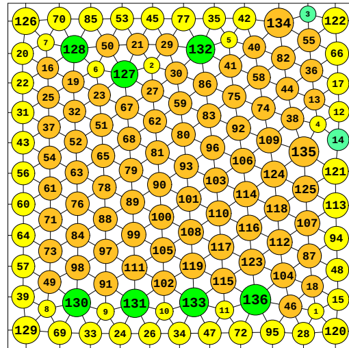
N = 136 136 circles in a square
