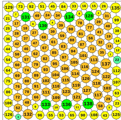
N = 138 138 circles in a square
