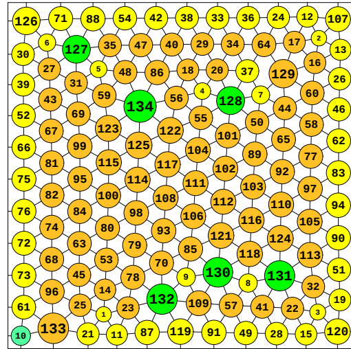
N = 134 134 circles in a square
