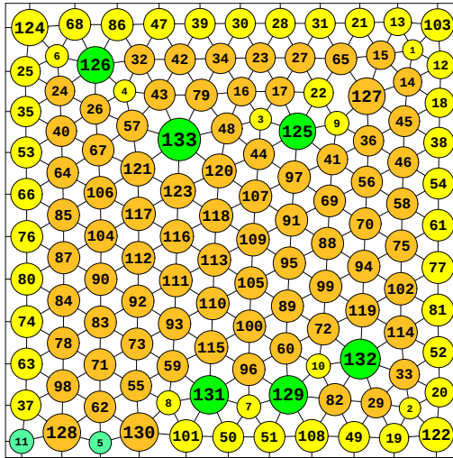
N = 133 133 circles in a square
