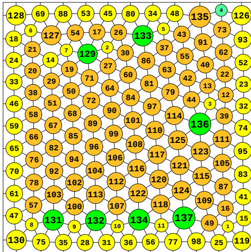
N = 137 137 circles in a square
