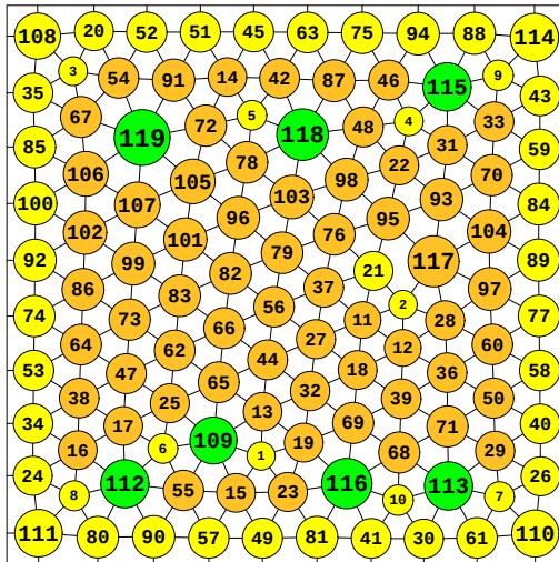
N = 119 119 circles in a square
