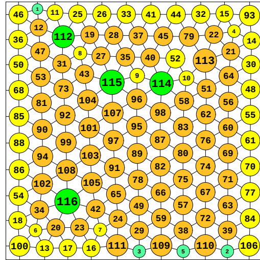
N = 116 116 circles in a square
