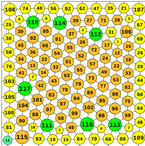
N = 117 117 circles in a square
