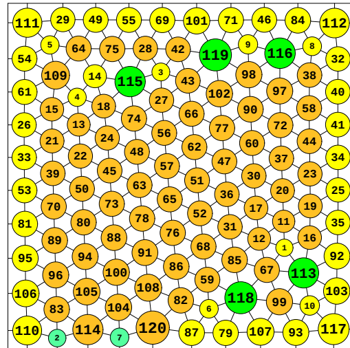
N = 120 120 circles in a square
