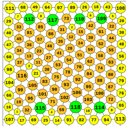
N = 118 118 circles in a square
