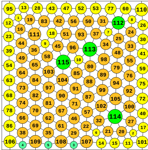
N = 115 115 circles in a square
