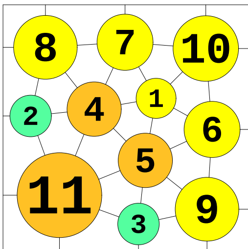
N = 11 11 circles in a square
