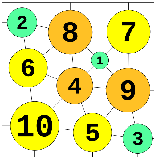
N = 10 10 circles in a square
