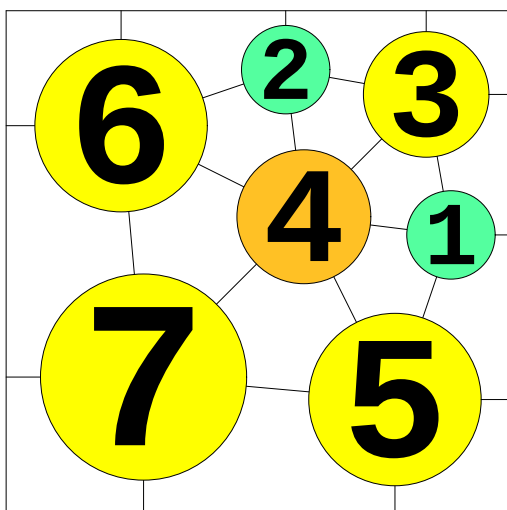
N = 7 7 circles in a square
