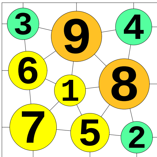
N = 9 9 circles in a square
