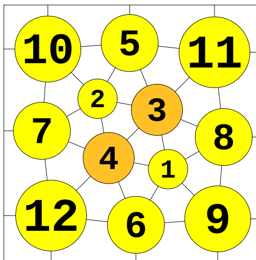
N = 12 12 circles in a square
