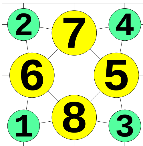
N = 8 8 circles in a square
