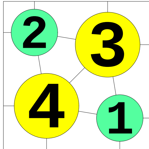
N = 4 4 circles in a square
