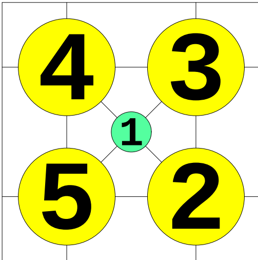
N = 5 5 circles in a square
