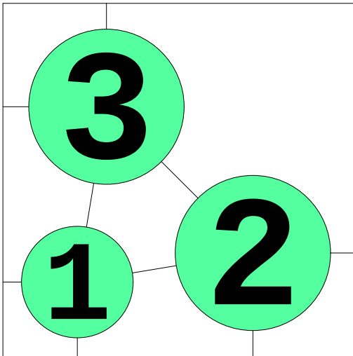
N = 3 3 circles in a square
