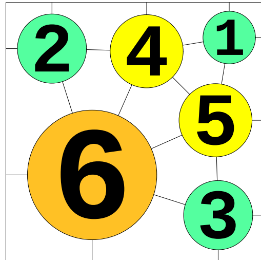
N = 6 6 circles in a square
