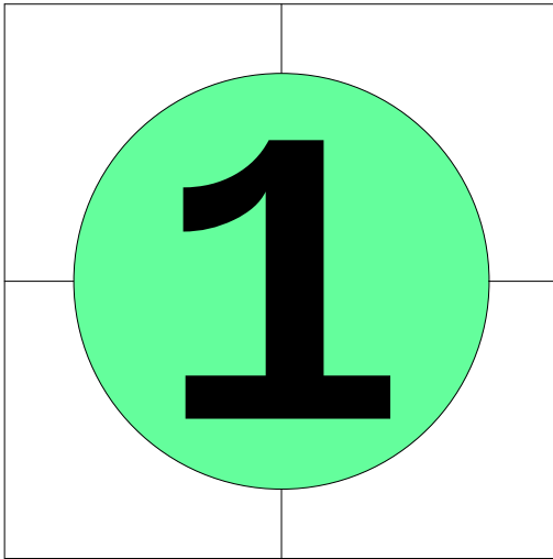
N = 1 1 circle in a square
