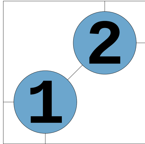
N = 2 2 circles in a square
